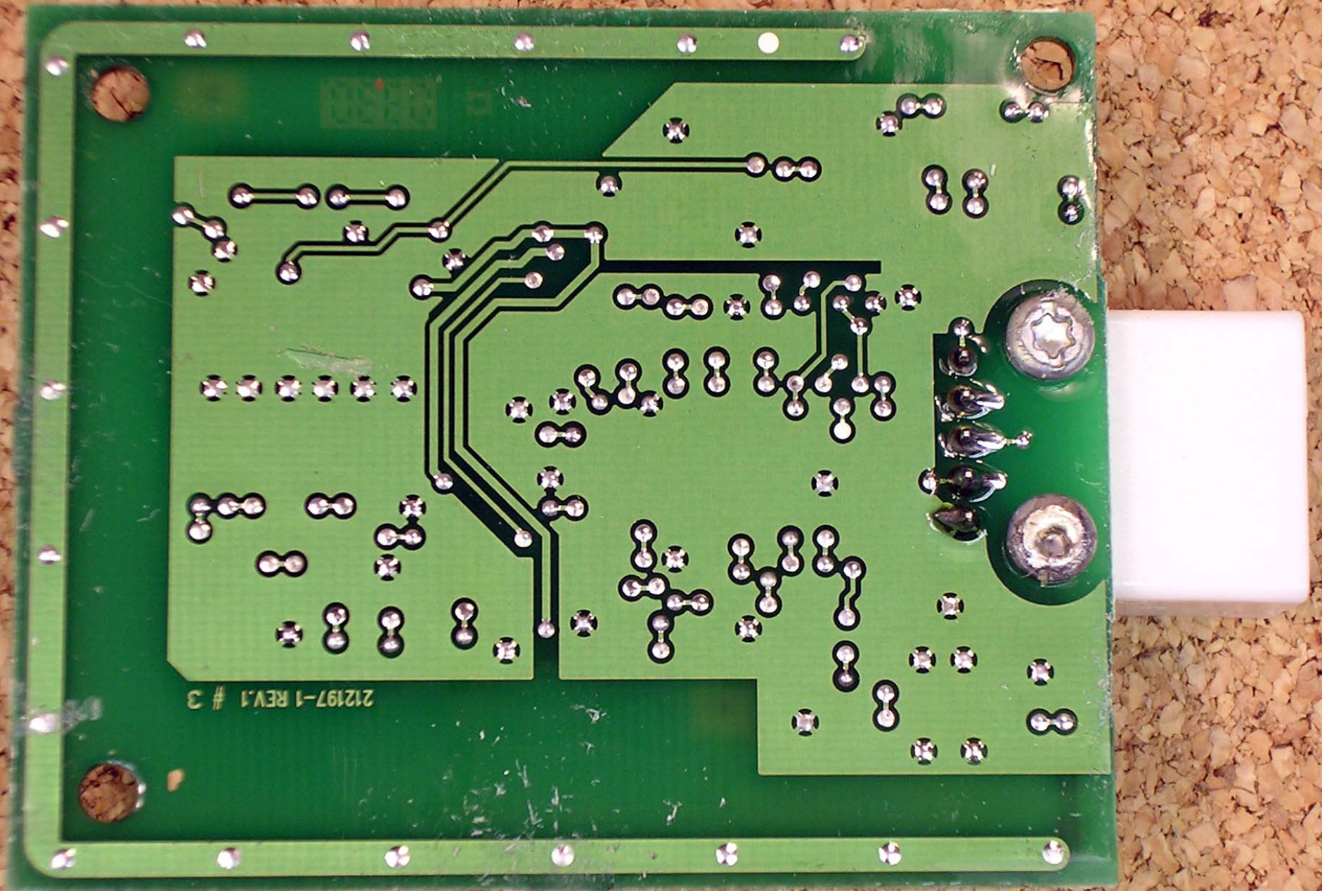
PCB (bottom)
