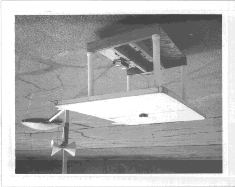
Figure 5.3. Close-up of the DUT on the open-site test table for worst case emissions at "fundamental".
