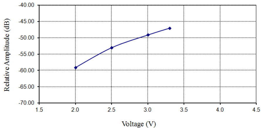
Figure 6.4. Relative emission at fundamental vs. supply voltage (cw). DUT tested with new 3.3 VDC battery when demonstrating compliance.
