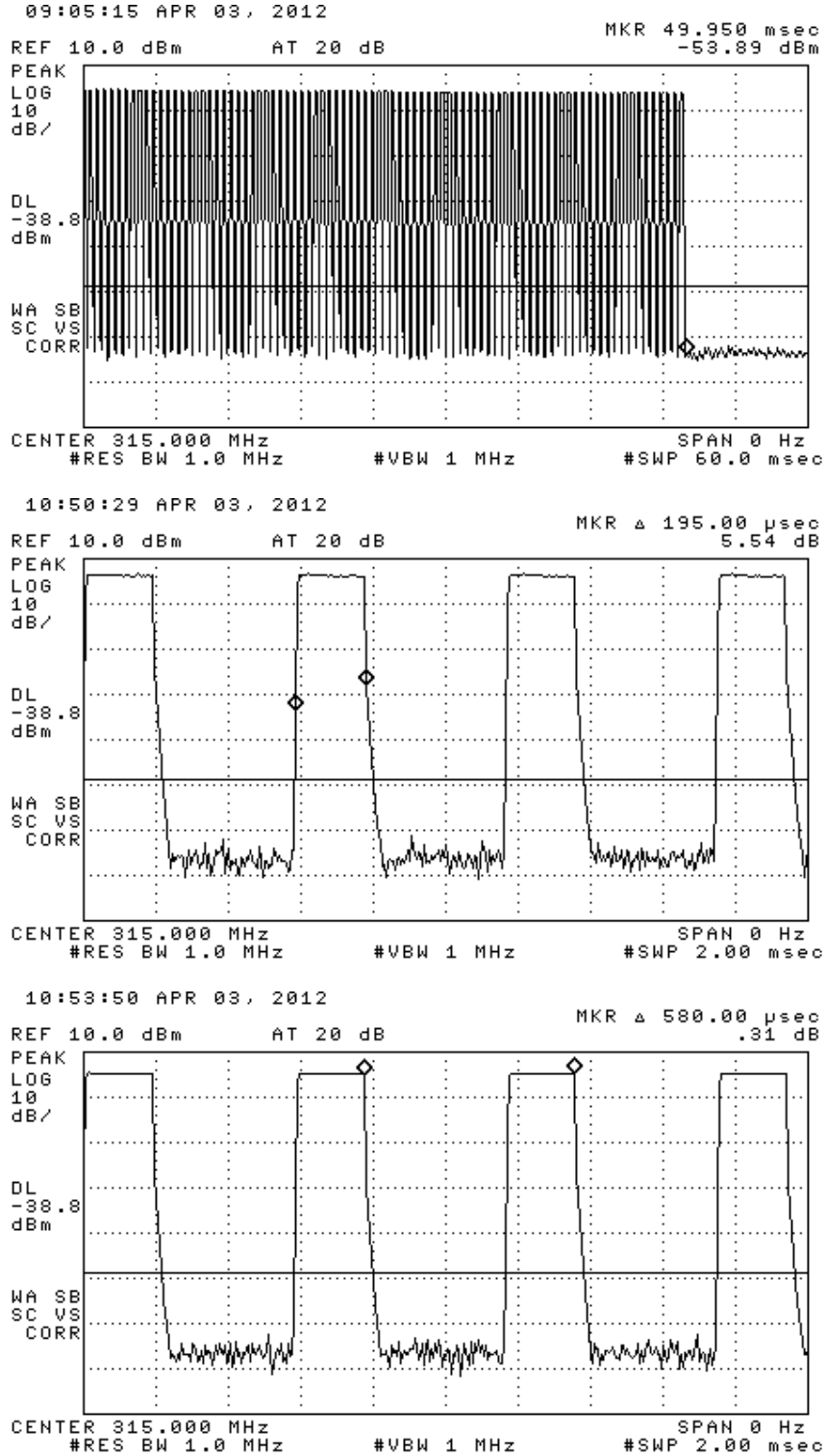
Figure 6.1(b). First frame encoding. (top) first frame length, (center) first frame pulse width, (bottom) first frame pulse period.
