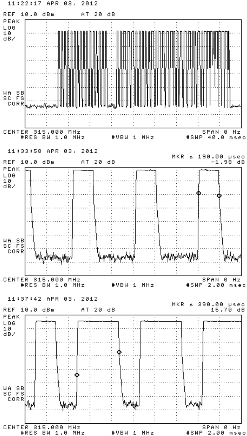
Figure 6.1 (c), Repeated PWM frame encoding. (top) complete frame, (center) PWM frame narrow bit width, (bottom) PWM frame wide bit width.
