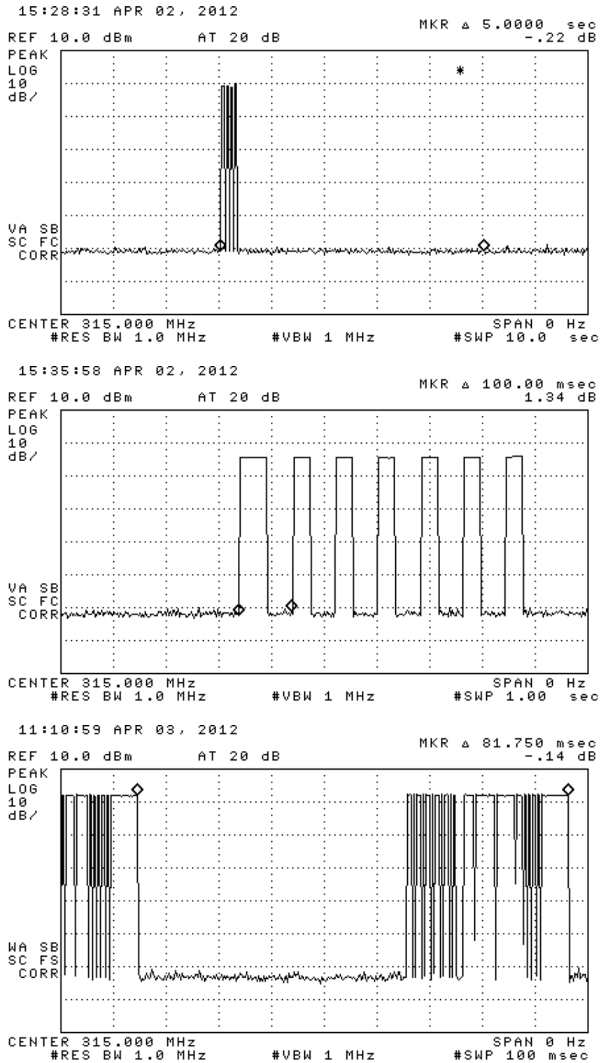
Figure 6.1(a). Transmission characteristics. (top) single button press transmission, (middle) first frame period, (bottom) repeated frames period
