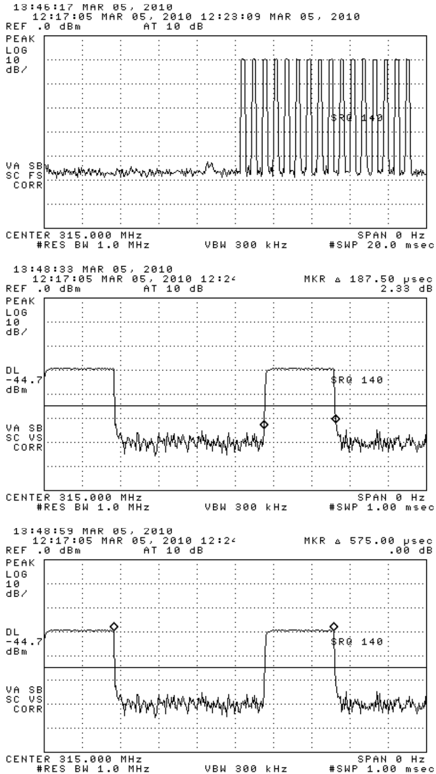
Figure 6.1(b). Transmission modulation characteristics. (top) wake packet, (center) wake pulse width, (bottom) wake pulse period.
