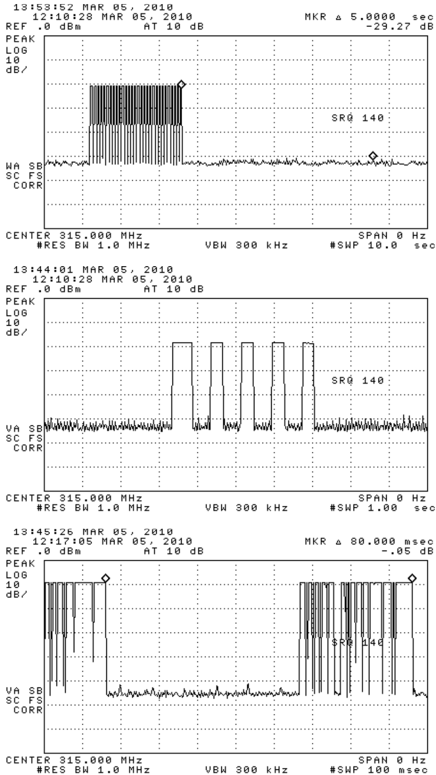
Figure 6.1(a). Transmission modulation characteristics. (top) 5 second button release turn off (center) expanded transmission, (bottom) transmission period.
