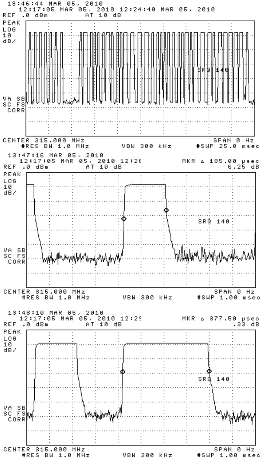
Figure 6.1(c). Transmission modulation characteristics. (top) complete Manchester data packet, (center) Manchester bit with, (bottom) Manchester bit period.
