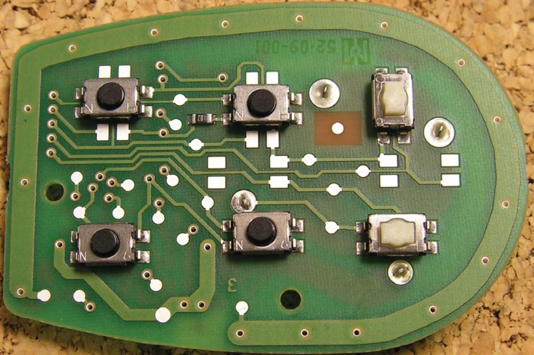
PCB (top)
