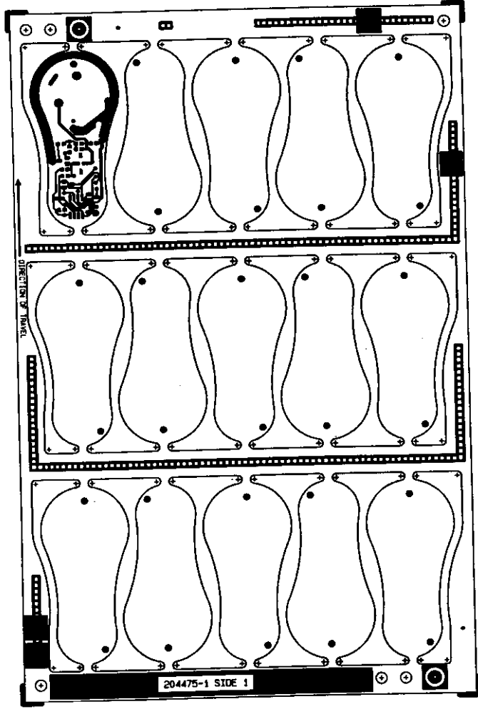
ARTWORK - CIRCUIT, TOP SIDE
