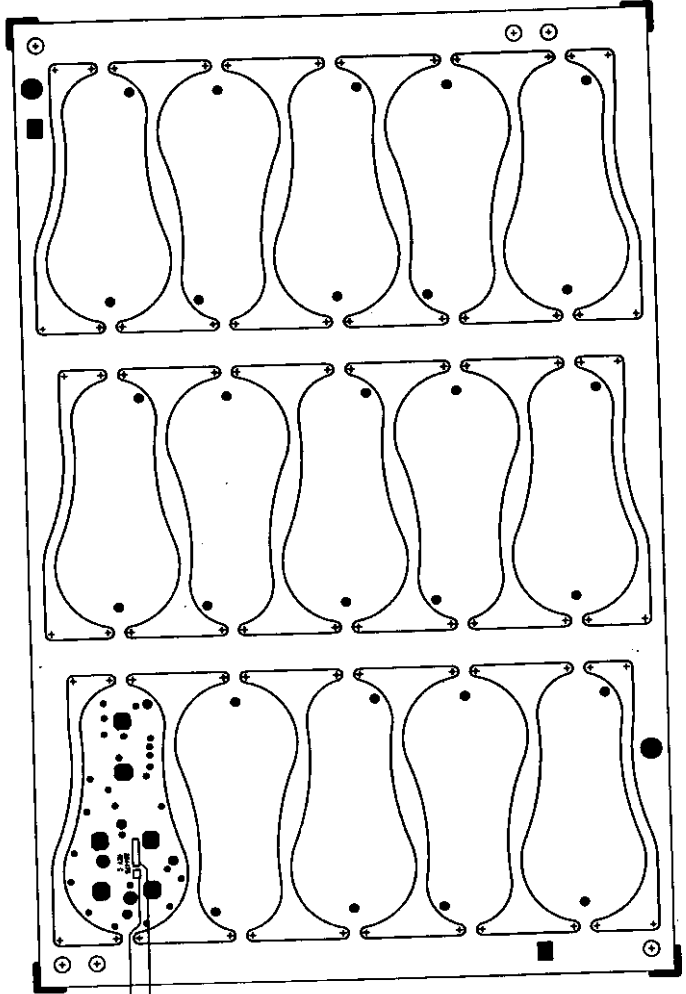
ARTWORK - SOLDER MASK, BOTTOM SIDE
