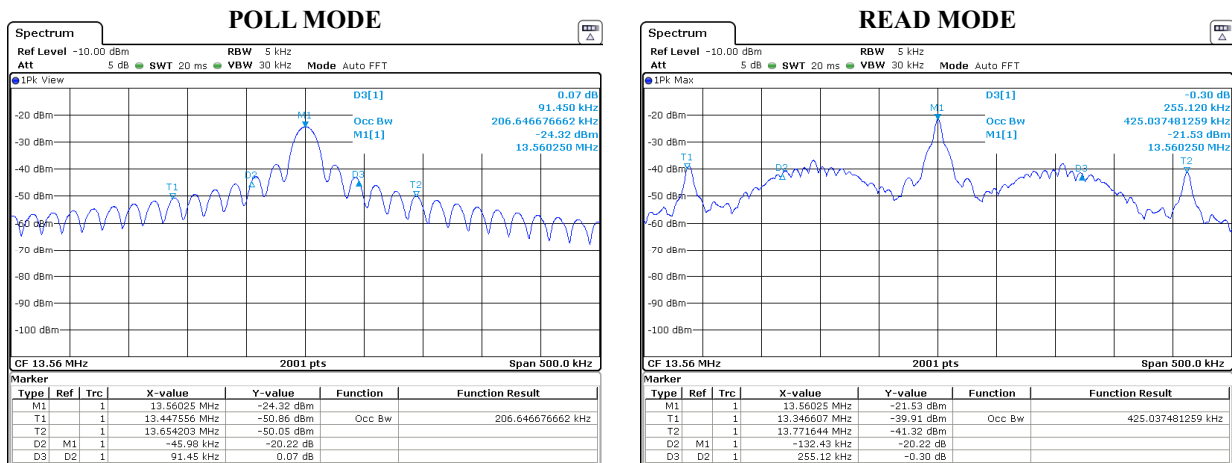
Figure 6: Intentional Emission Bandwidth.
