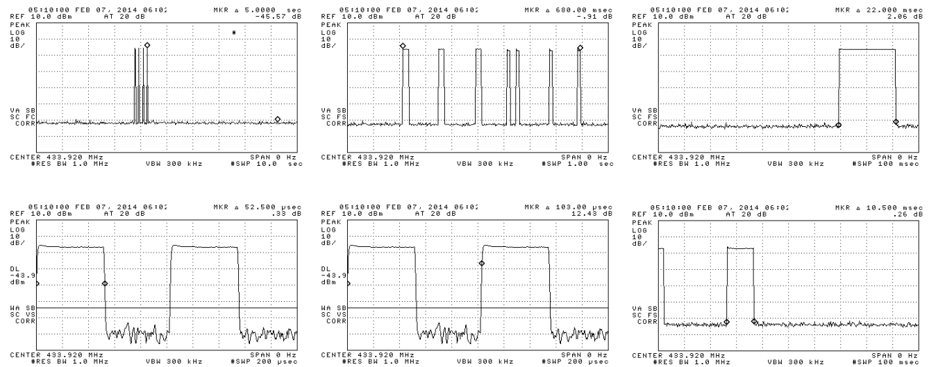
Figure 5(a): Pulsed Emission Characteristics (Duty Cycle).
