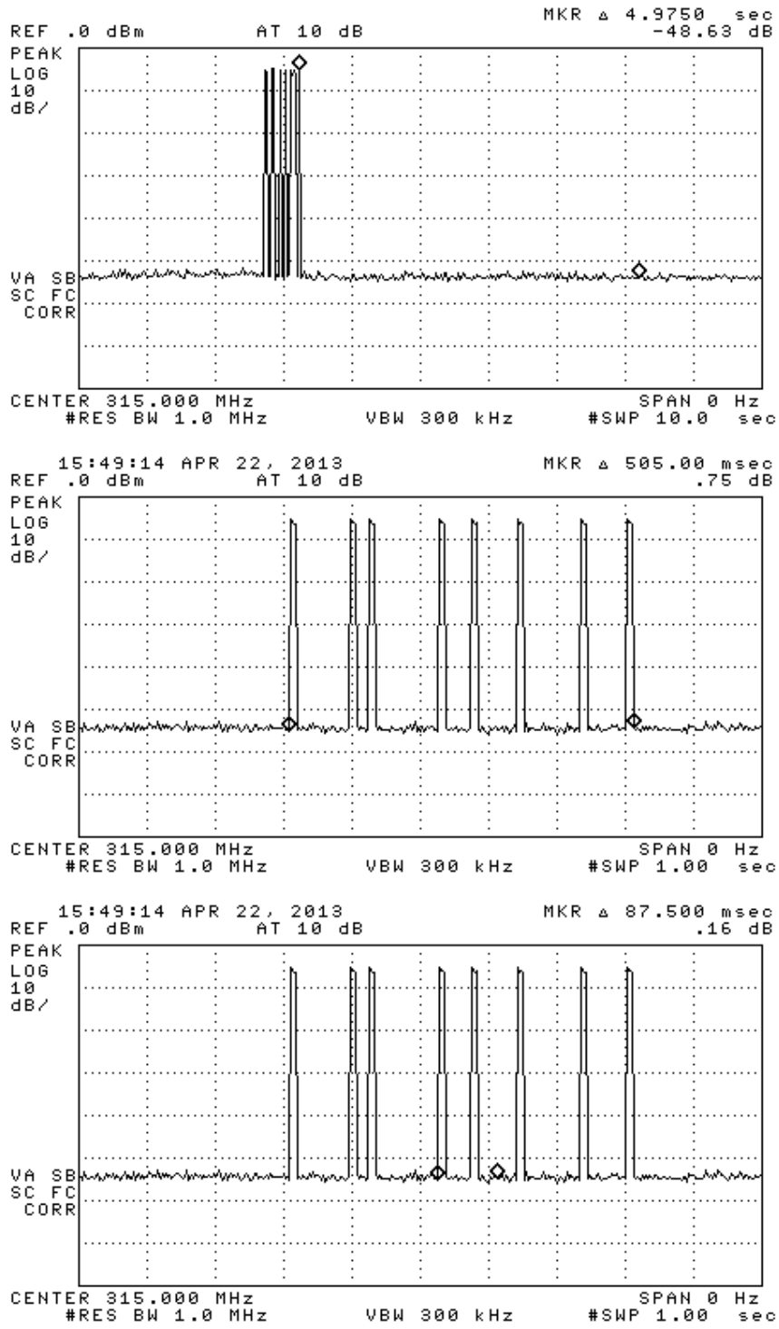
Figure 6.1(a). LF Actuated Transmission characteristics. (top) single transmission, (center) expanded transmission, (bottom) max of two frames per 100 ms window.
