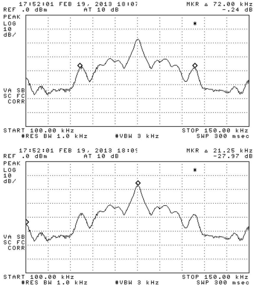
Figure 6.2. Measured emission bandwidth of the DUT (pulsed).
