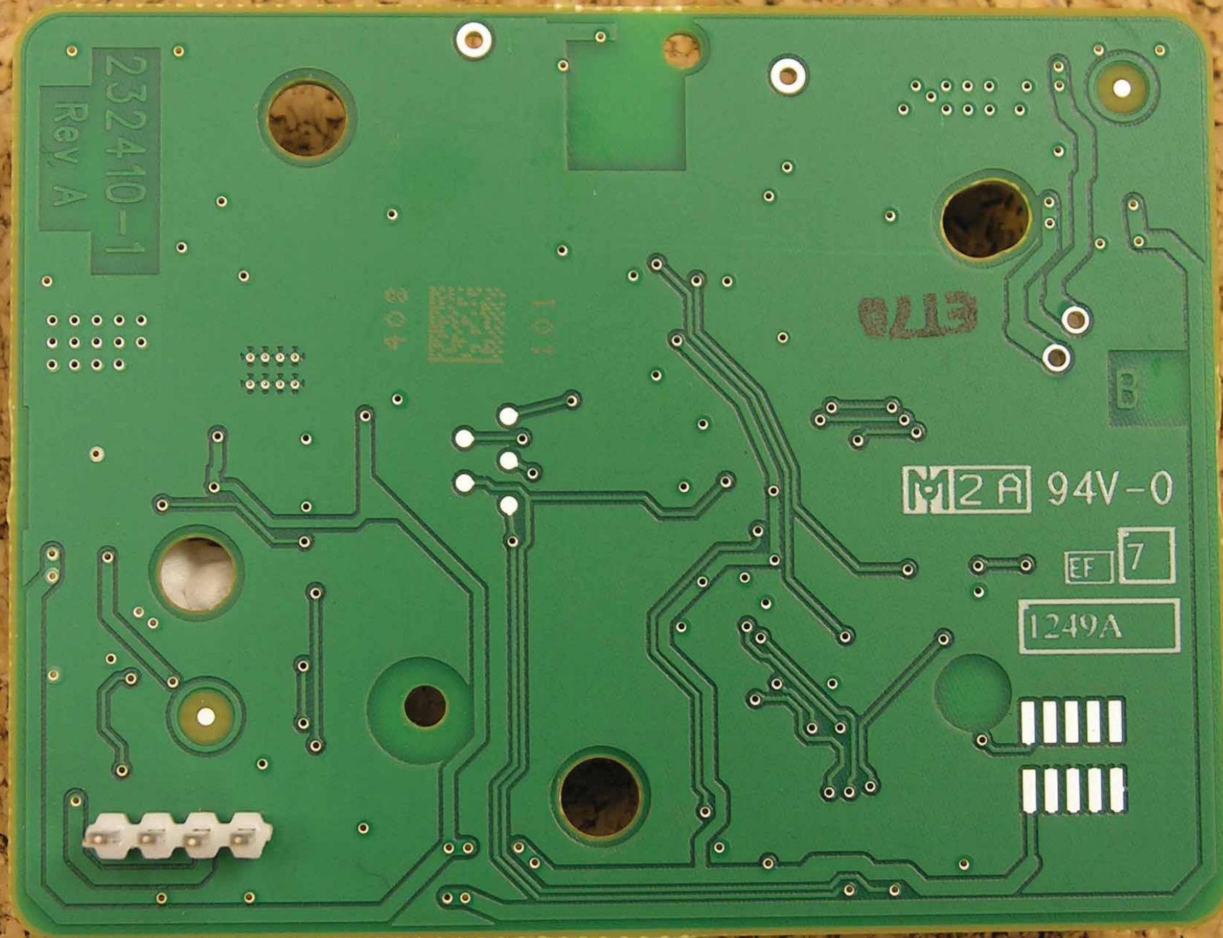
PCB (bottom)
