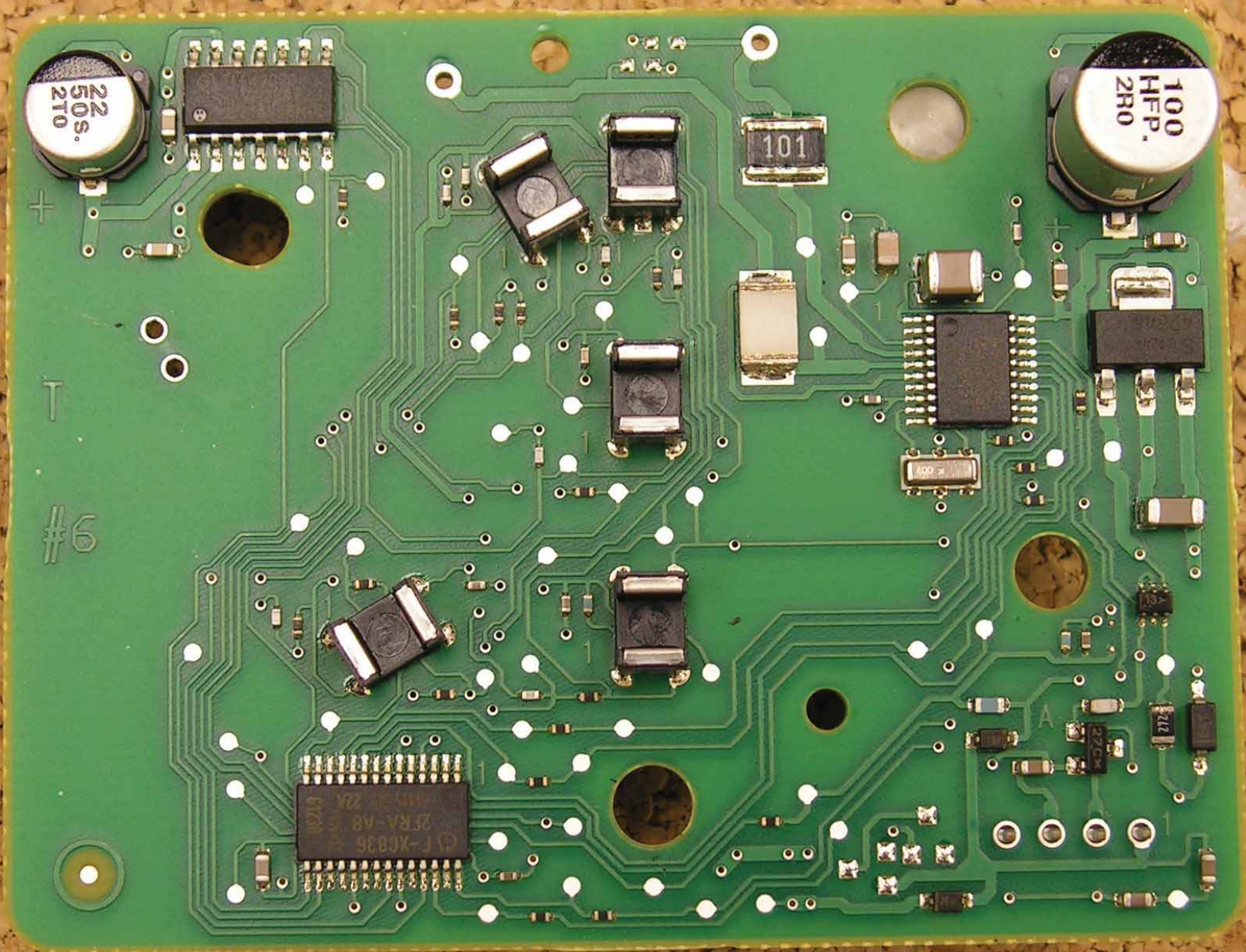
PCB (top)
