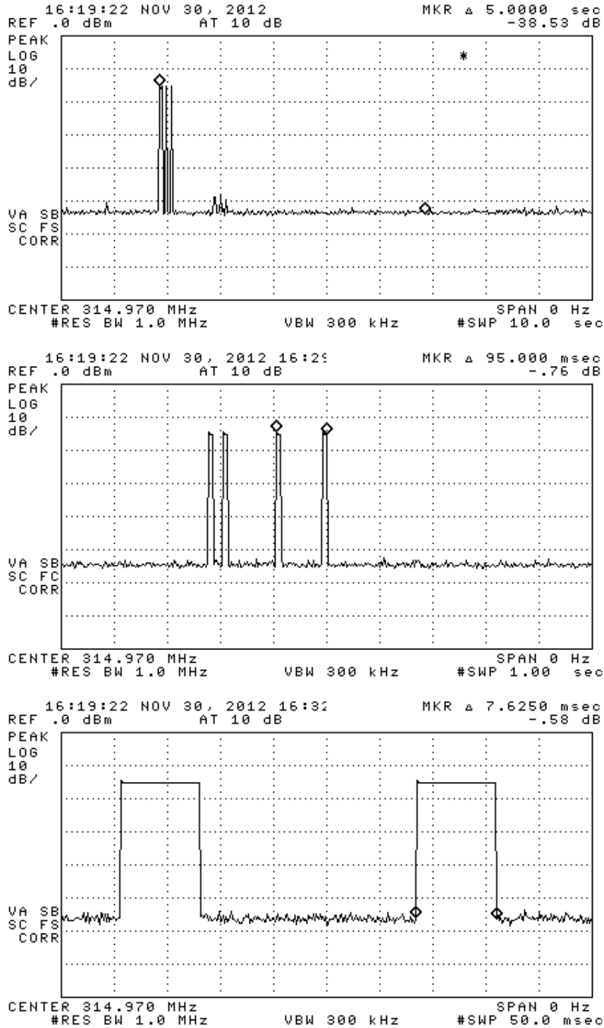
Figure 6.1(a). Manually Actuated Transmission characteristics. (top) complete transmission, (center) expanded transmission, (bottom) expanded frame.
