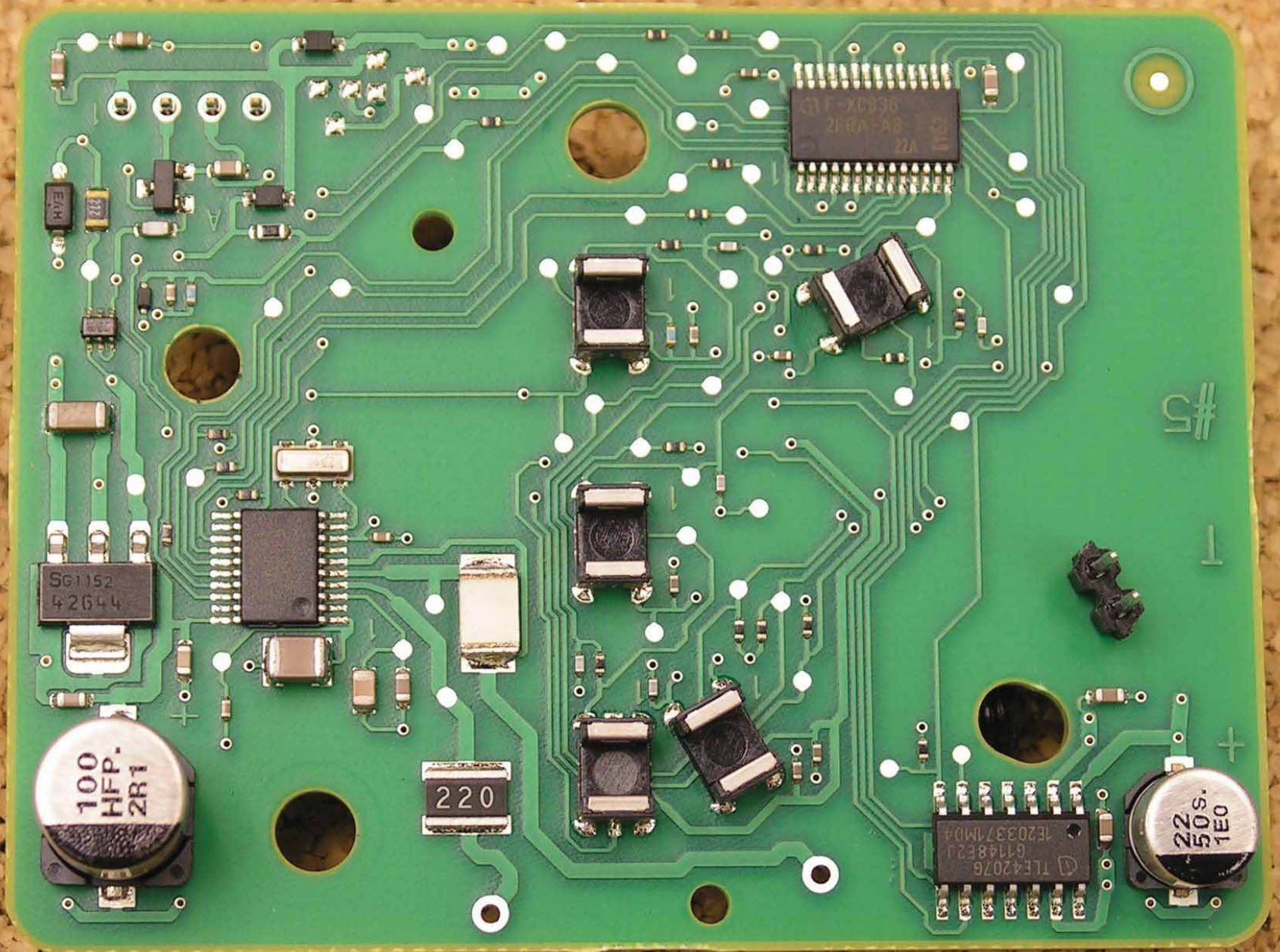
PCB (top)
