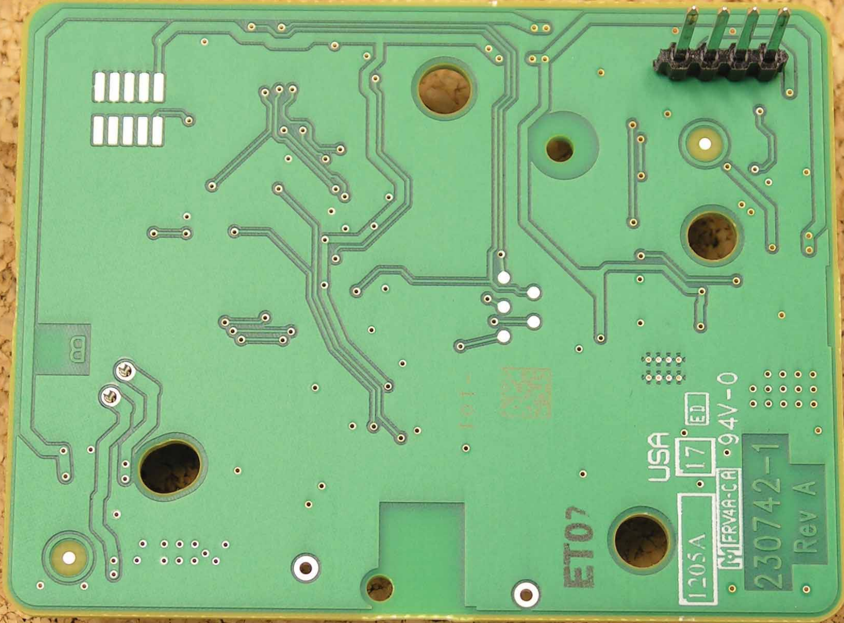
PCB (bottom)
