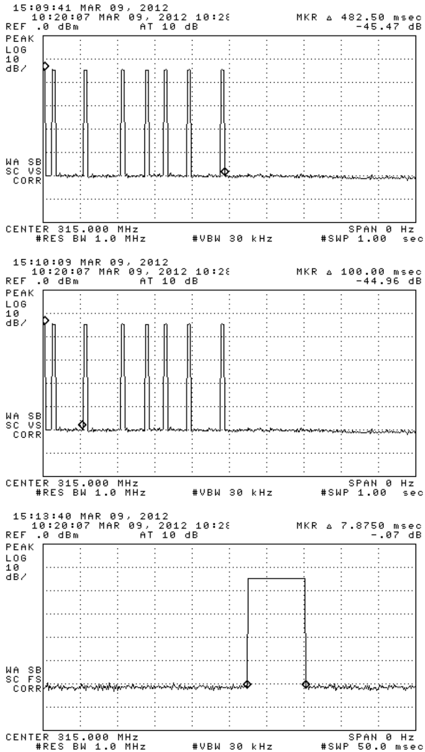
Figure 6.1. FSK Transmission modulation characteristics. (top) complete transmission, (center) two frames / 100 ms, (bottom) single FSK frame length
