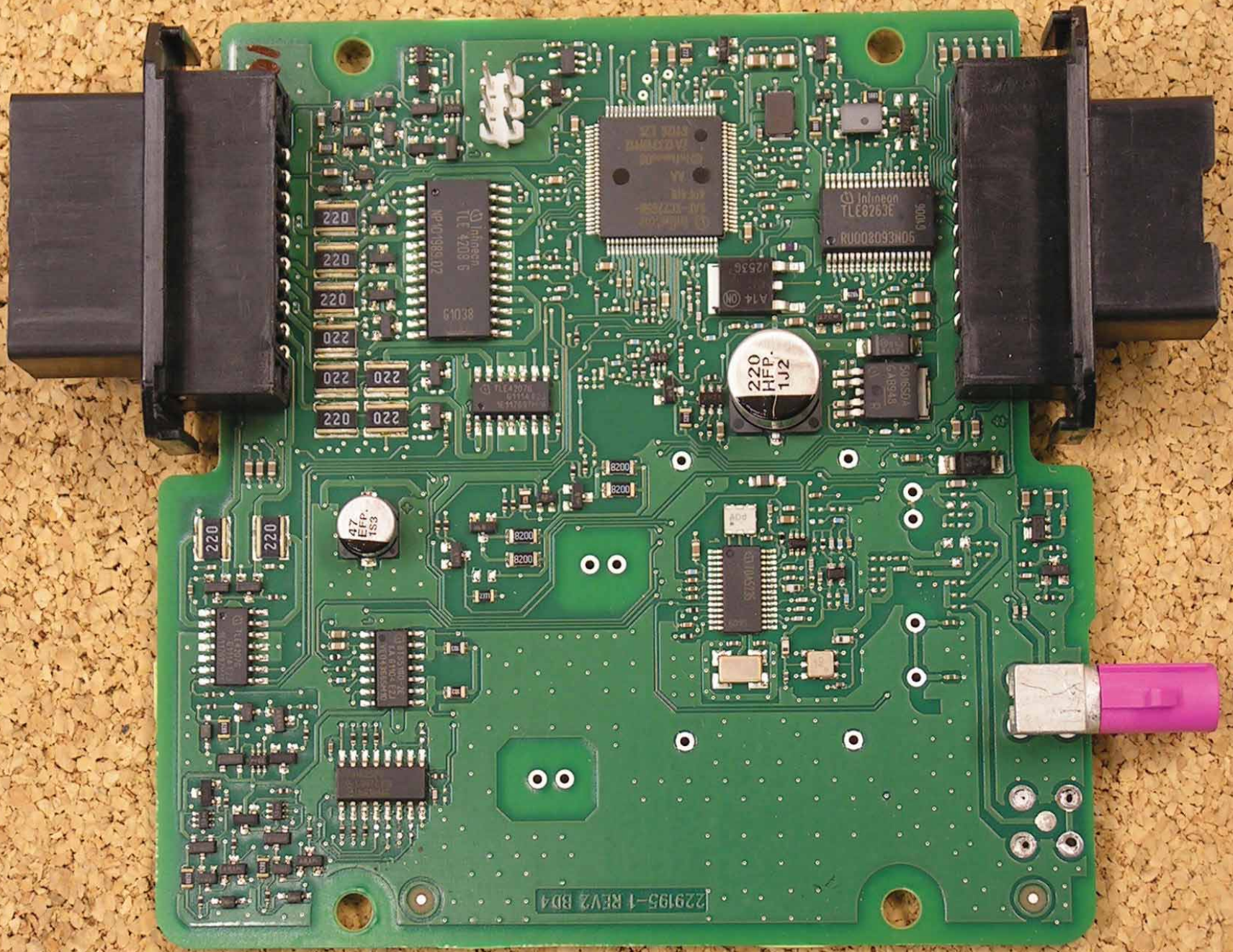
PCB (top)
