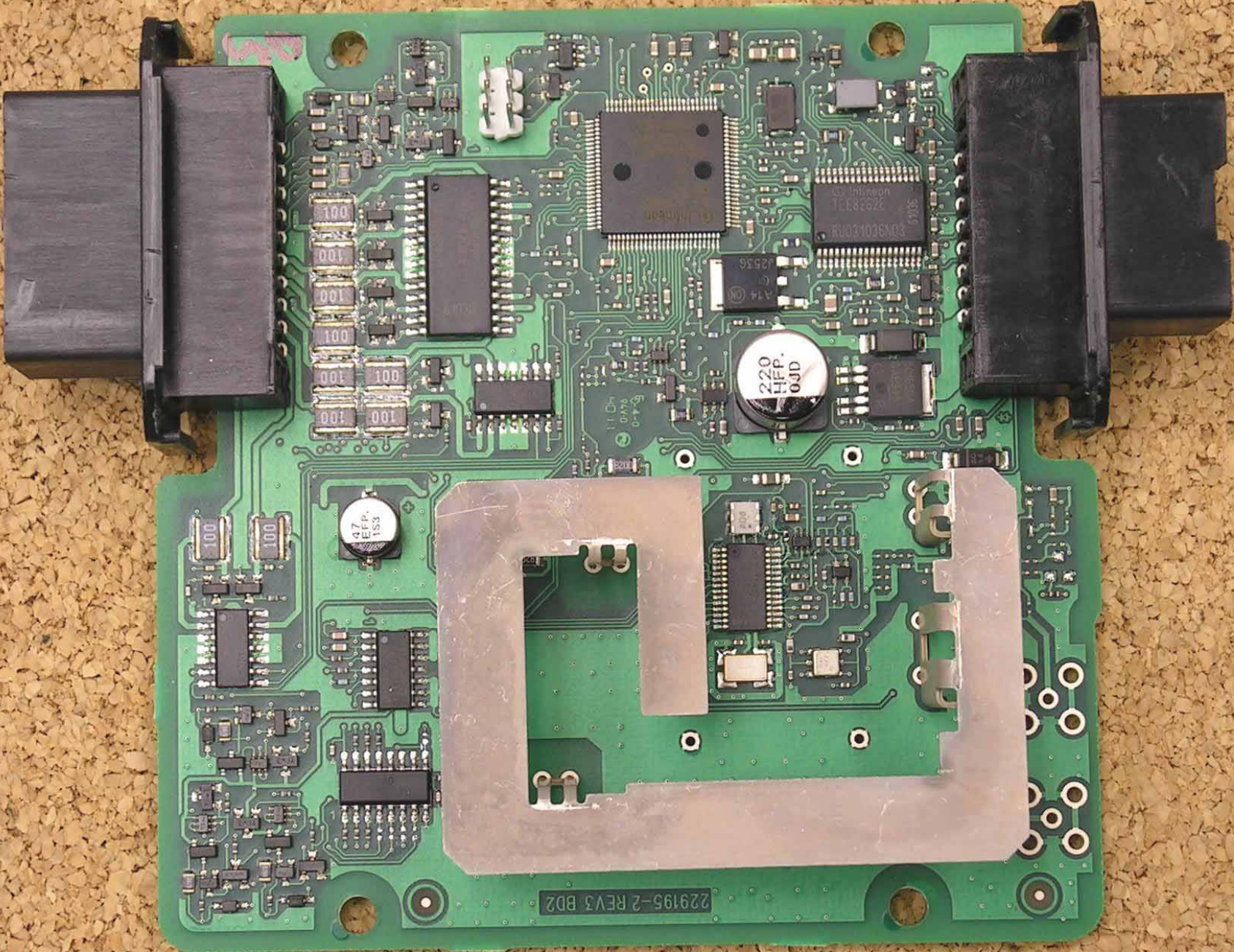
PCB (top)
