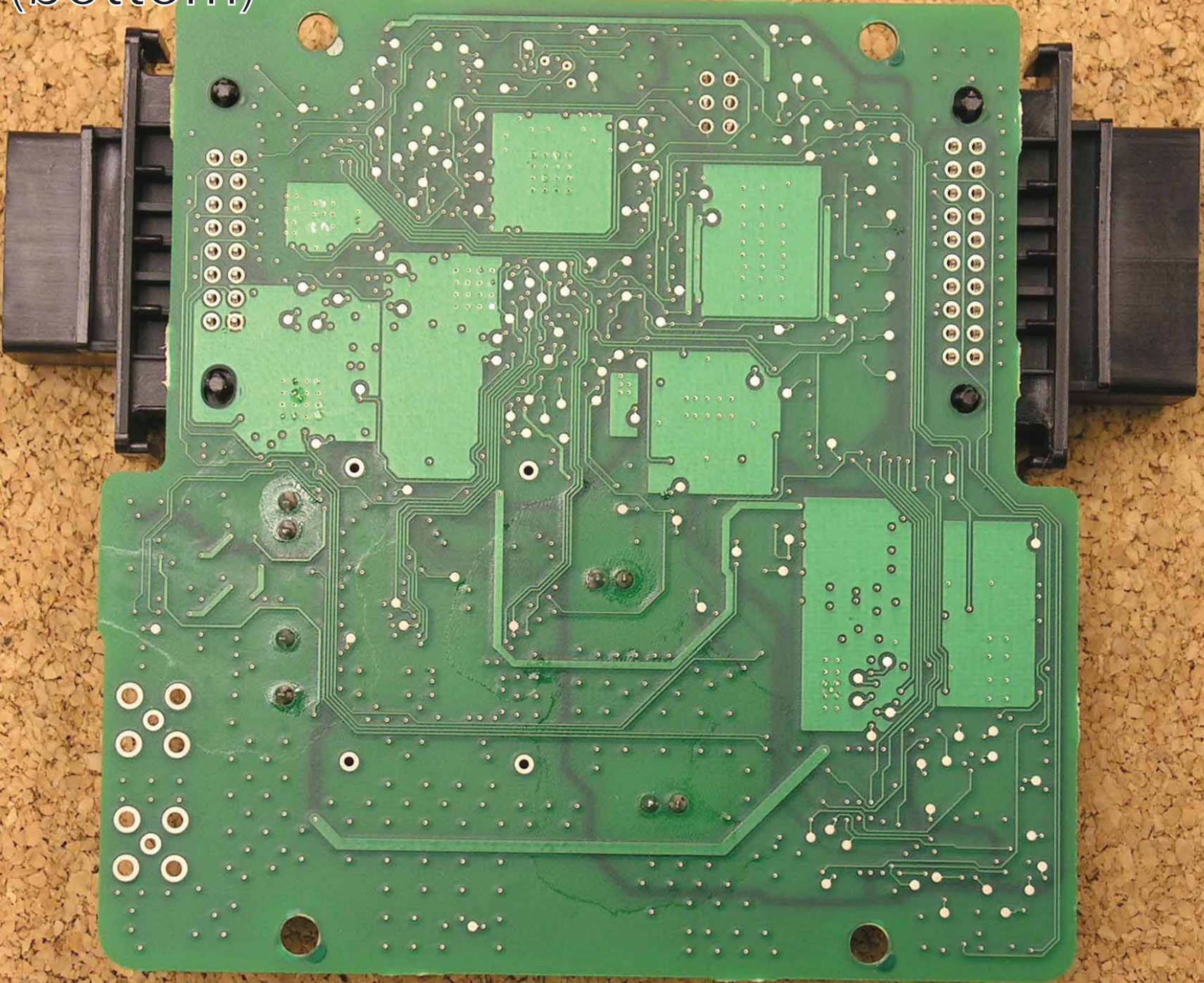
PCB (bottom)
