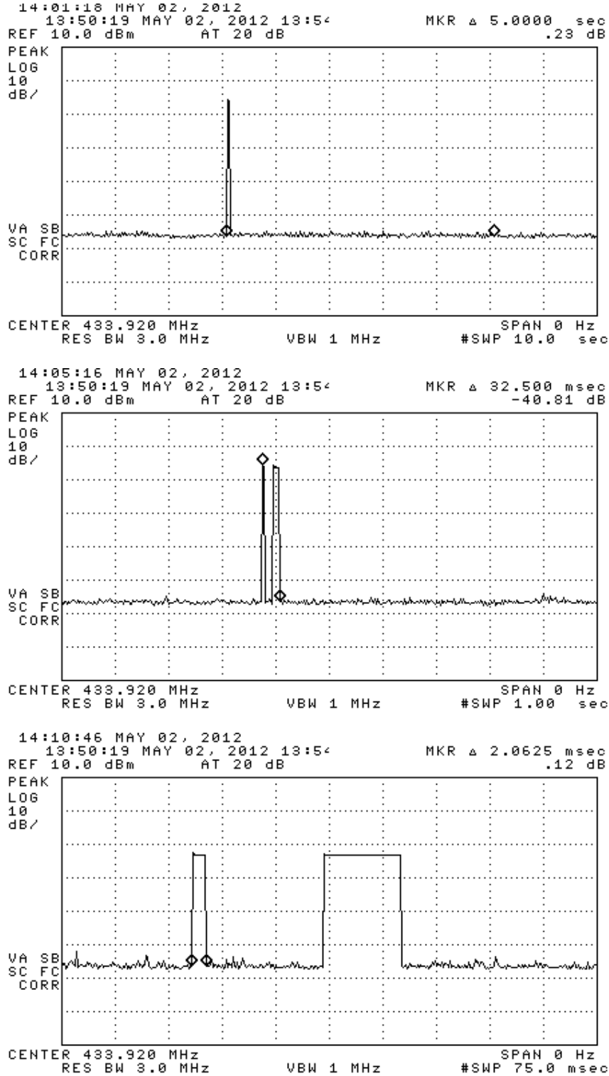
Figure 6.1(c). Passive Entry / Passive Start (FSK) Mode. (top) complete transmission, (center) expanded transmission, (bottom) first frame length.
