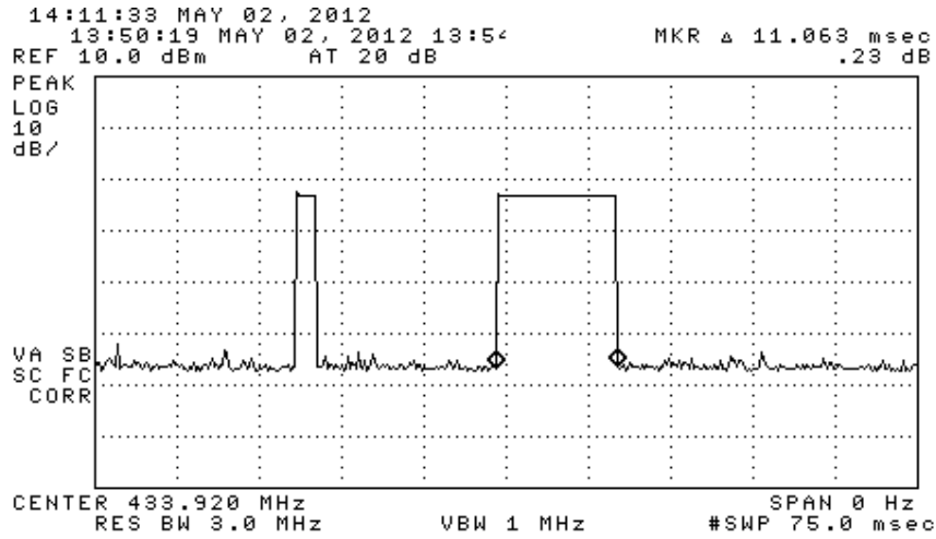
Figure 6.1(d). Passive Entry / Passive Start (FSK) Mode. (top) complete transmission, (center) expanded transmission, (bottom) second frame length.
