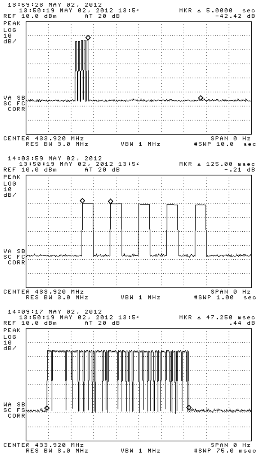
Figure 6.1(a). RKE mode transmission characteristics. (top) complete transmission, (center) expanded transmission, (bottom) expanded frame.
