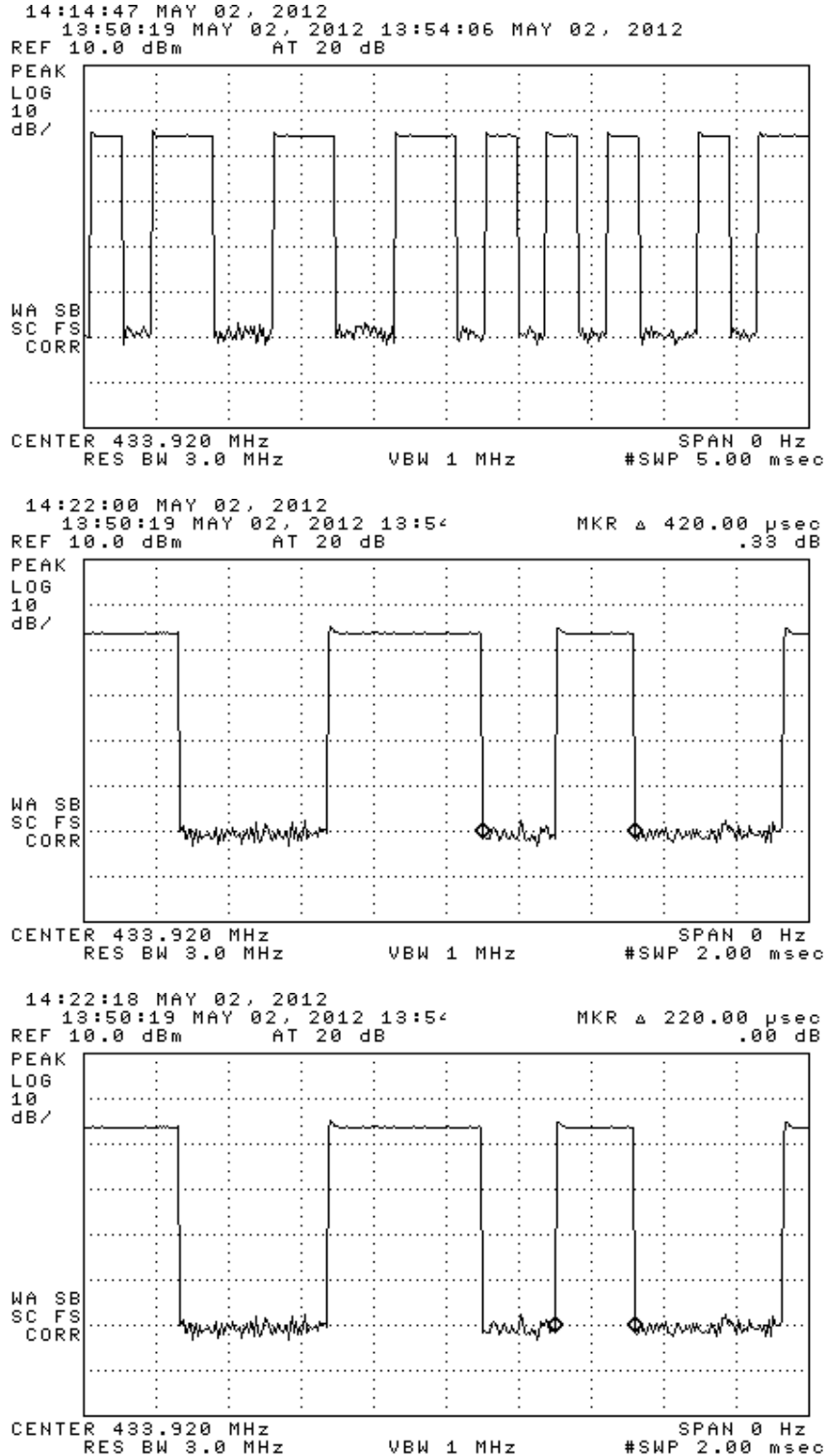
Figure 6.1(b). RKE mode transmission characteristics. (top) complete frame, (center) Manchester period, (bottom) Manchester pulse width.
