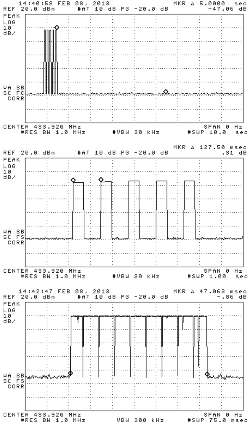
Figure 6.1(a). Transmission modulation characteristics. (top) single manual activation, (center) expanded transmission, (bottom) expanded frame.
