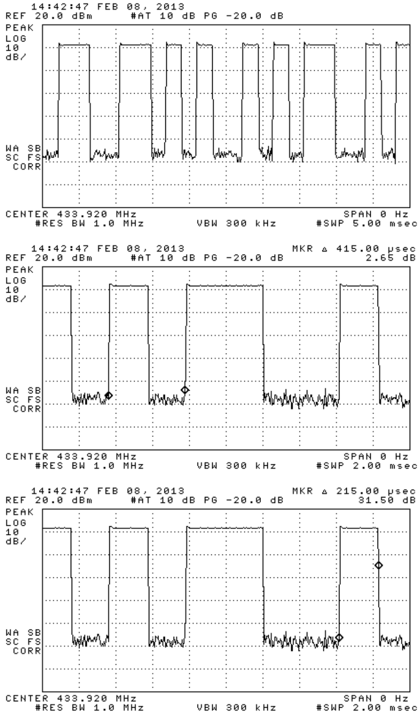
Figure 6.1(b). Transmission characteristics. (top) Manchester frame encoding, (center) bit period, (bottom) bit width.
