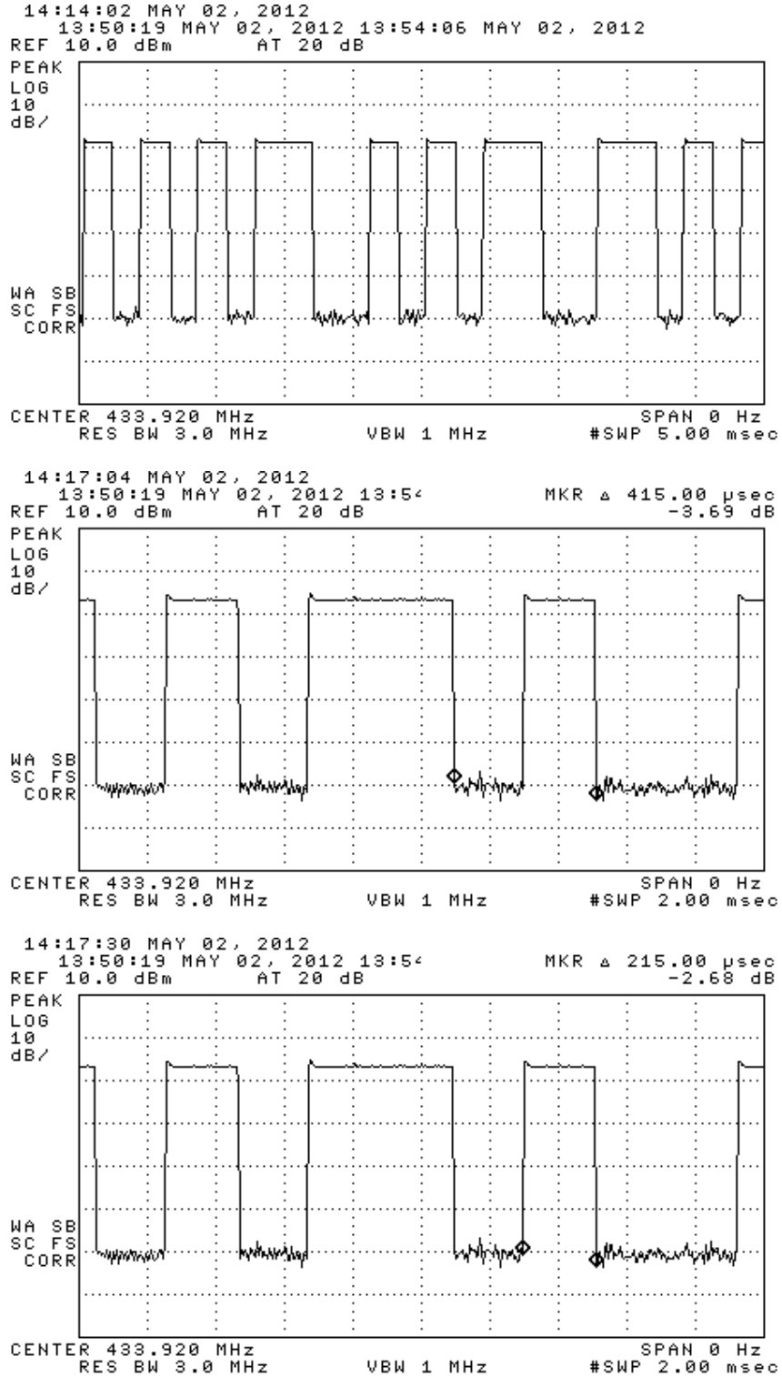
Figure 6.1(b). Transmission modulation characteristics. (top) expanded frame, (center) Manchester period, (bottom) Manchester pulse-width.
