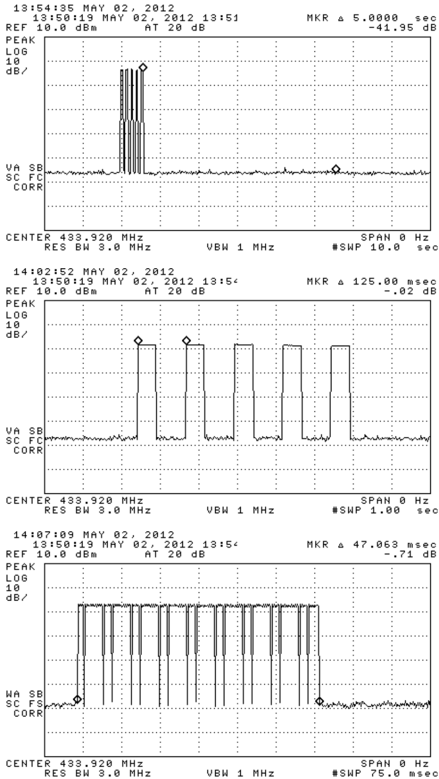
Figure 6.1(a). Transmission modulation characteristics. (top) complete transmission from single button press, (center) expanded transmission, (bottom) expanded frame.
