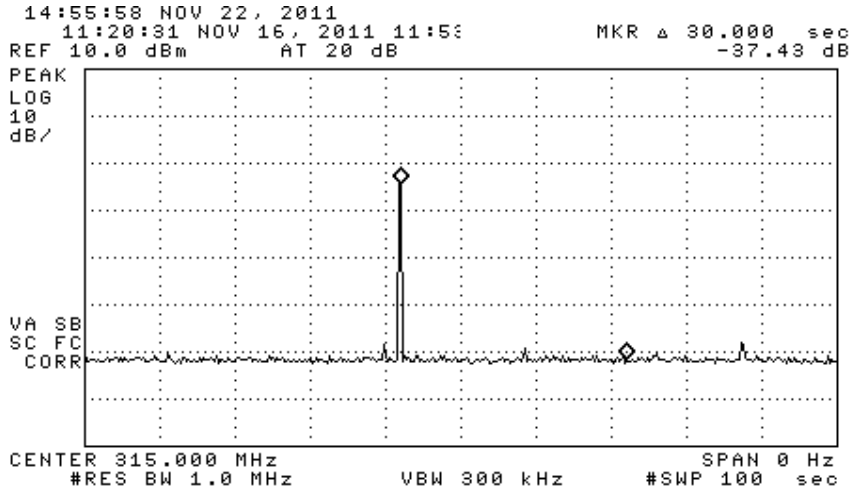
Figure 6.1(b). Drive Mode Transmission characteristics. One transmission every 180 seconds - same duty as LF actuated mode above.
