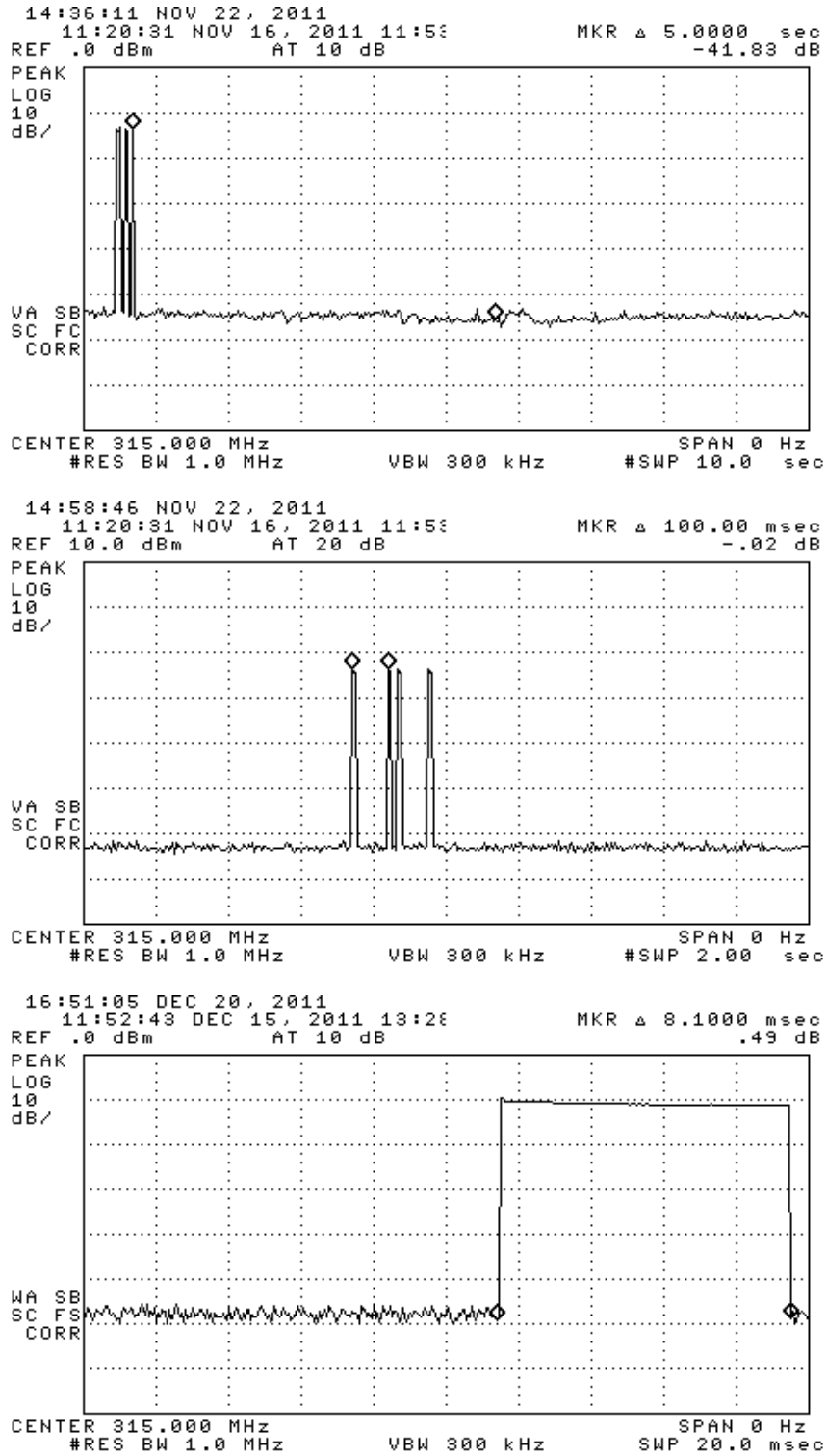
Figure 6.1(a). LF actuated transmission characteristics. (top) single activation, (center) transmission frames – two per 100 ms window, (bottom) single frame.
