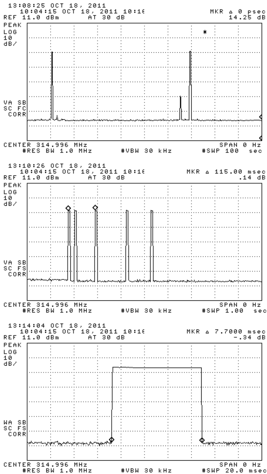
Figure 6.1(a). Drive Mode transmission characteristics. (top) periodic transmission, (center) expanded transmission, (bottom) single FSK frame.
