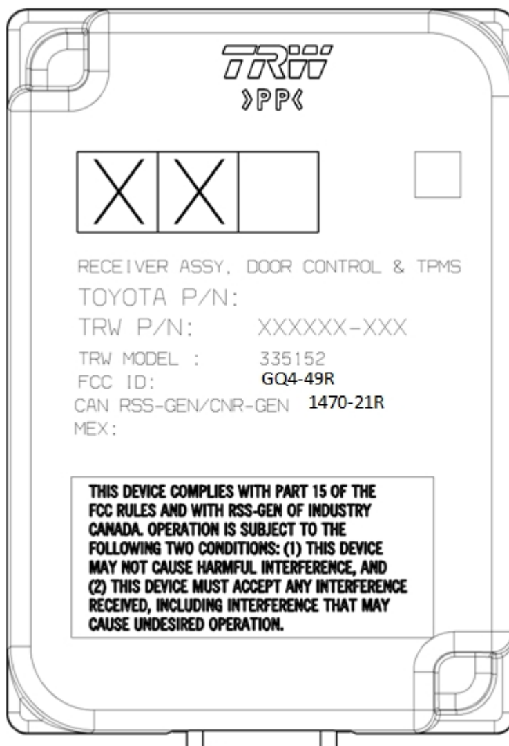
Figure 1 – Placement Drawing
