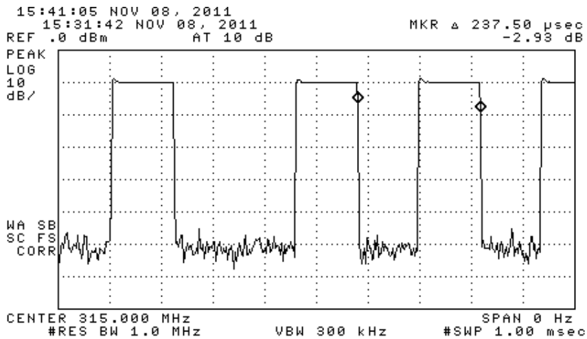
Figure 6.1(b). Frame characteristics. (top) Manchester encoded frame (center) bit width, (bottom) bit period.
