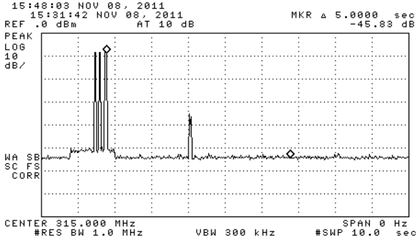
Figure 6.1(c). Lear Mode Transmission. Manual activation by LF interrogation, 3 frame response.
