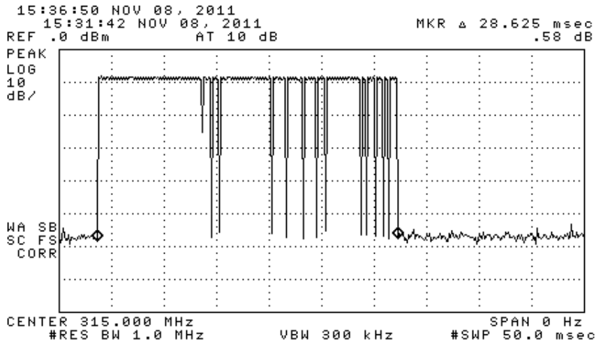
Figure 6.1(a). Drive Mode Transmission characteristics. (top) periodic transmission (other spurs not from DUT), (center) expanded transmission, (bottom) expanded frame.
