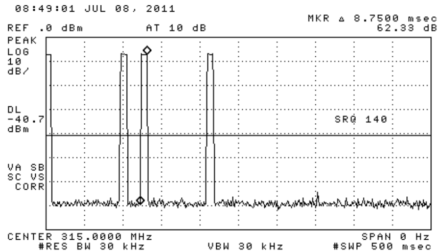
Figure 6.1(a). LF Activated / Stage 1 FSK Transmission characteristics. (top) complete transmission, (center) transmission window, (bottom) frame length.
