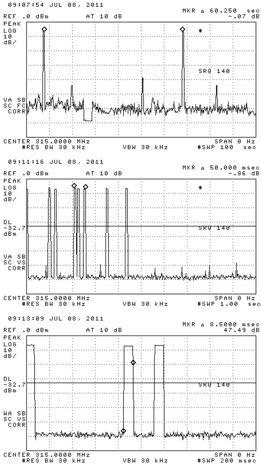
Figure 6.1(c) Stage 3 (Normal Periodic) Transmission characteristics. (top) periodic transmission, (center) worst case frames in 100 ms window, (bottom) single FSK frame length.
