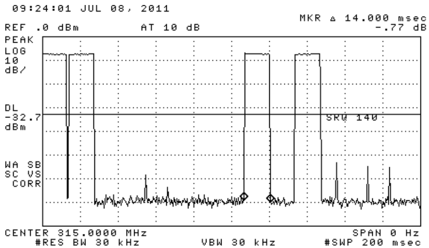
Figure 6.1(b). Stage 2 Transmission characteristics. (top) complete set of 8 transmissions, (center) expanded frames completed in less than 500 ms, (bottom) expanded single FSK frame.
