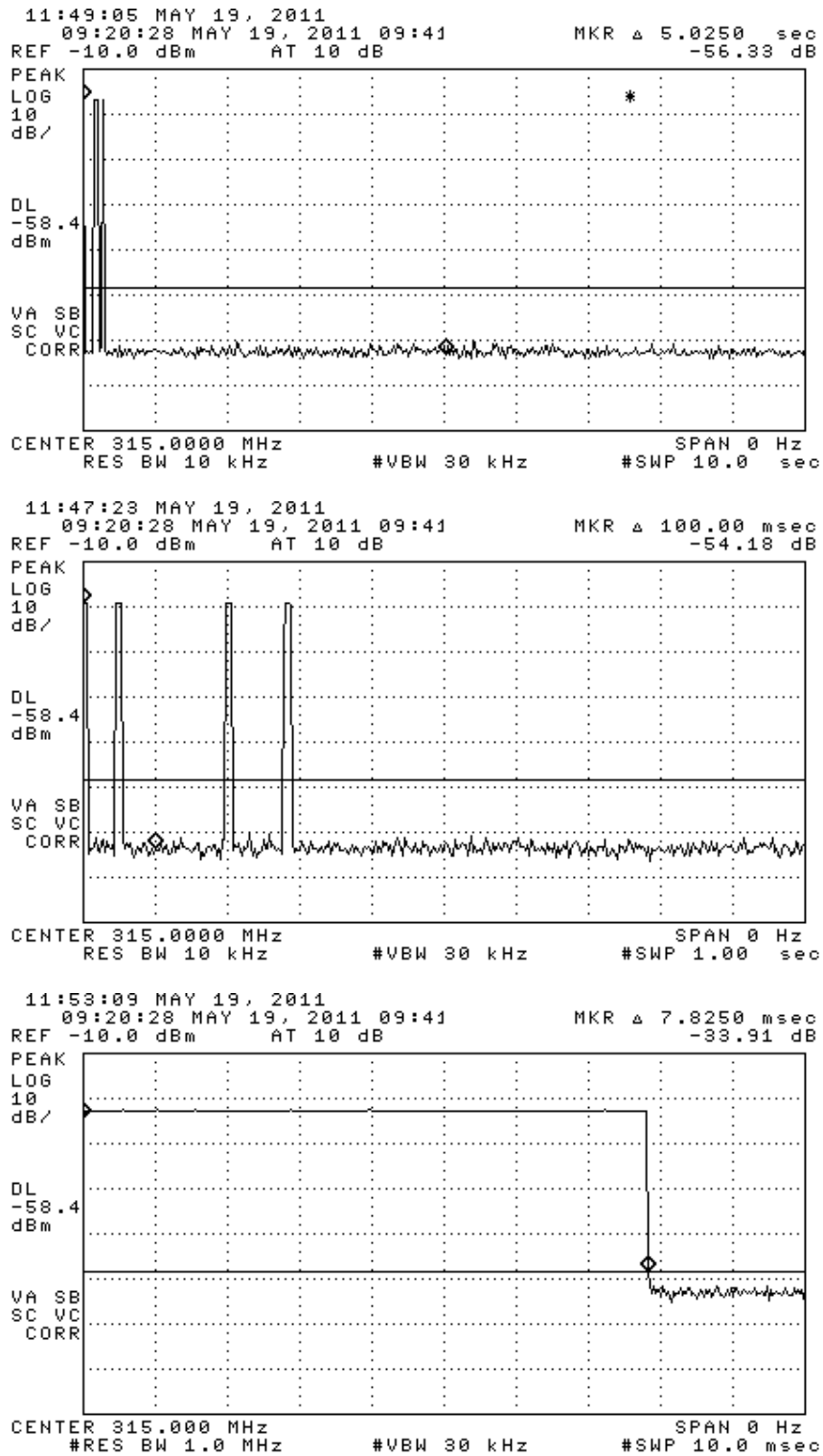
Figure 6.1. Transmission modulation characteristics. (top) complete transmission, (center) expanded transmission, (bottom) expanded FSK frame.
