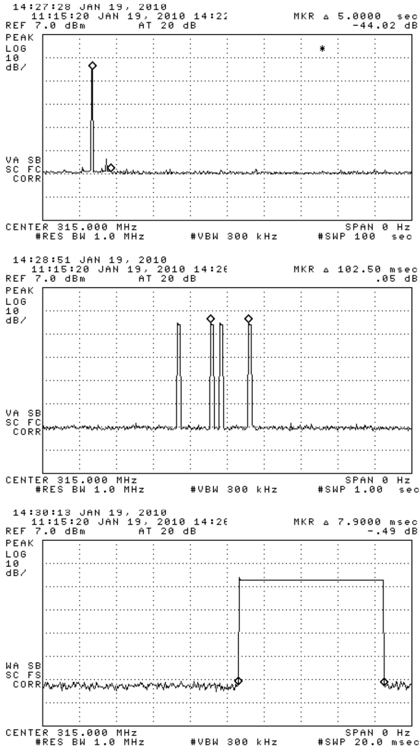
Figure 6.1. Transmission modulation characteristics. (top) one transmission (same for both rolling and LF activated mode), (center) expanded transmission, (bottom) expanded word.
