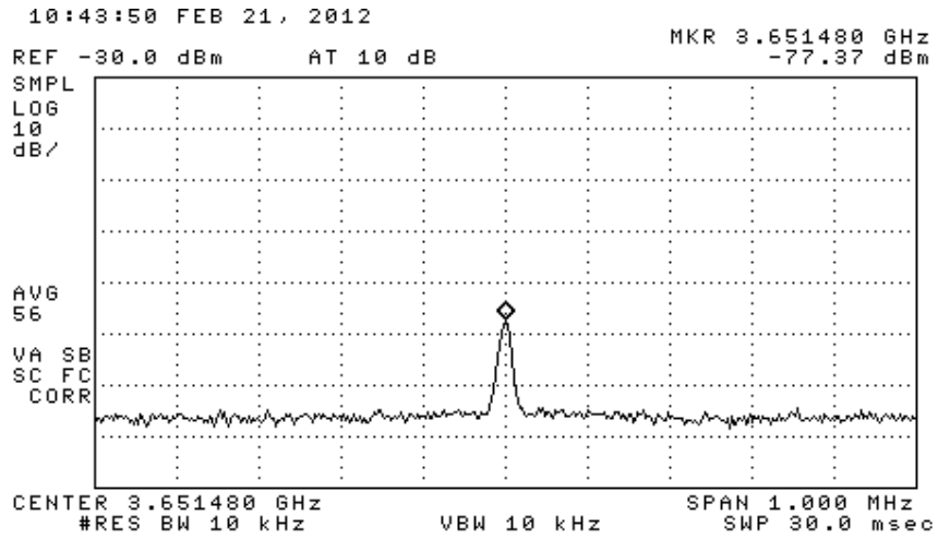
Figure 6.3. Example VCO emission at 10 cm distance, 10 kHz RBW.
