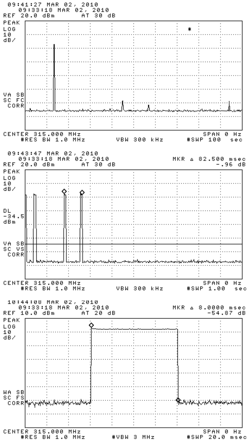
Figure 6.1. Transmission modulation characteristics. (top) transmission after LF interrogation, (center) expanded transmission, (bottom) expanded word.
