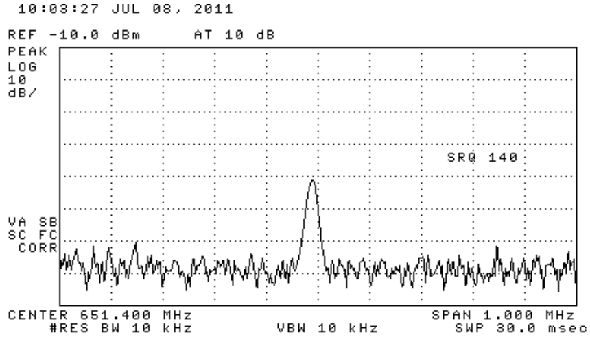
Figure 6.3. Receiver LO emission(s) - relative.
