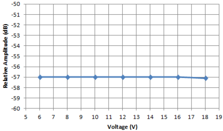
Figure 6.4. Relative emission vs. supply voltage.
