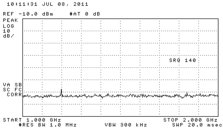
Figure 6.2. Emissions measured at 3 meters in chamber, 1000-2000 MHz. (emission at 1200 MHz is background)
