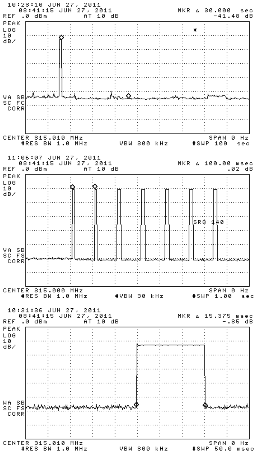
Figure 6.1(a). Periodic transmission modulation characteristics. (top) complete transmission, (center) expanded transmission, (bottom) single expanded FSK frame.
