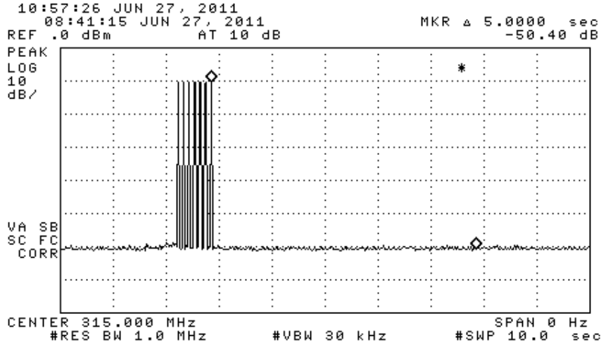
Figure 6.1(b) LF activated single transmission modulation. (Same frames as periodic above.)
