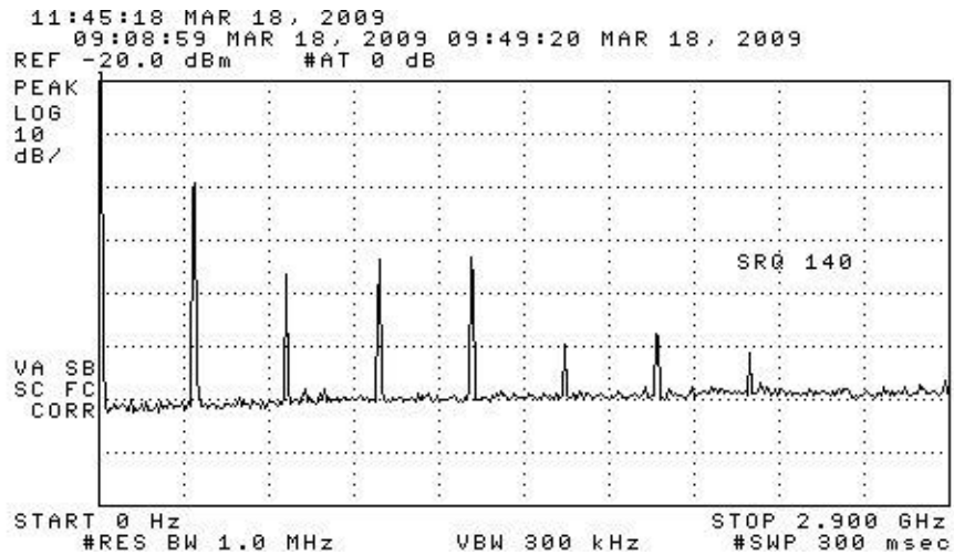
Figure 6.2. Emission spectrum of the DUT (pulsed emission).
