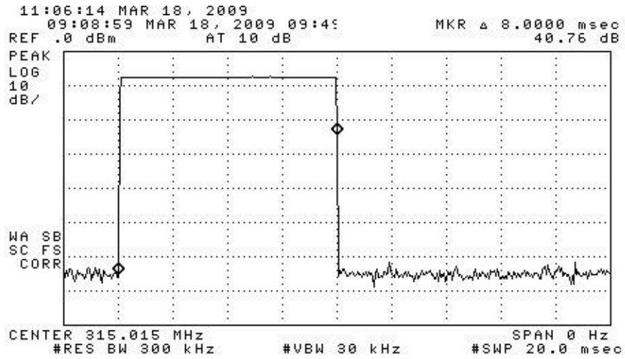
Figure 6.1(a). Transmission modulation characteristics. FSK word length.
