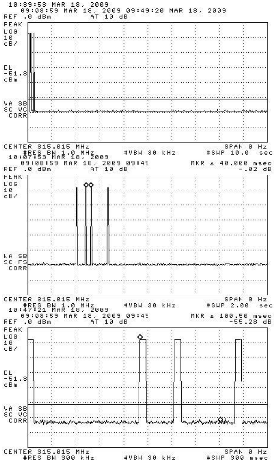
Figure 6.1(a). Transmission modulation characteristics. (top) complete transmission, (center) expanded transmission, (bottom) four words in transmission.
