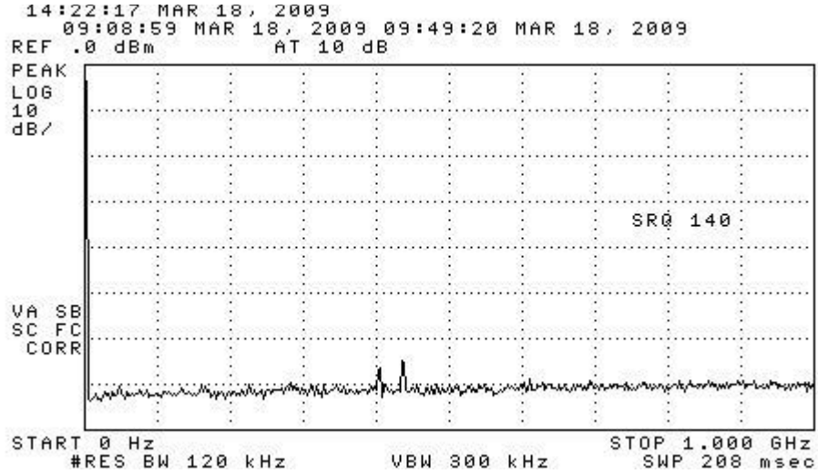
Figure 6.1. Emissions measured at 3 meters in chamber, 0-1000 MHz.
