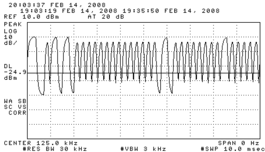
Figure 6.1. Transmission modulation characteristics. (top)
