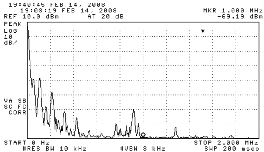
Figure 6.2. Emission spectrum of the DUT. (top) Spectrum, (bottom) Background The amplitudes are only indicative (not calibrated).
