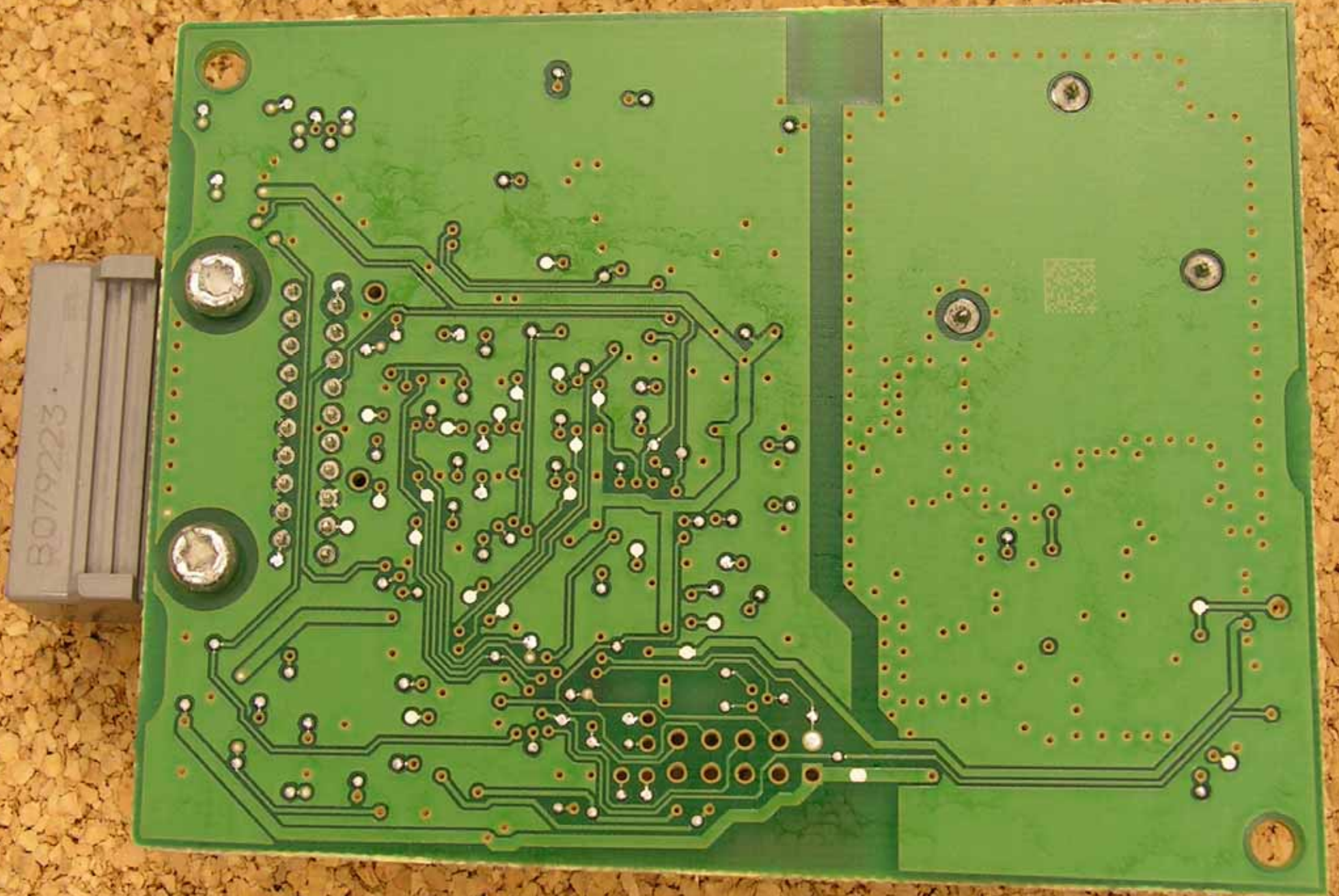
PCB (bottom)
