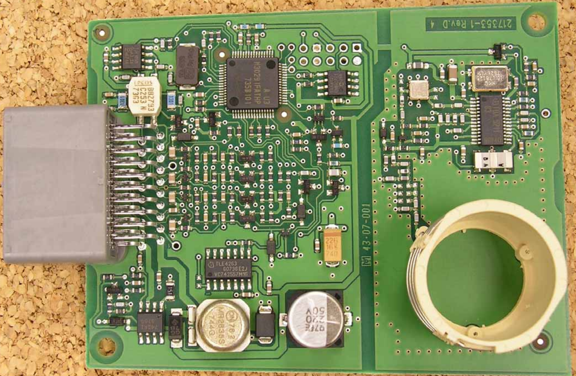
PCB (top)
