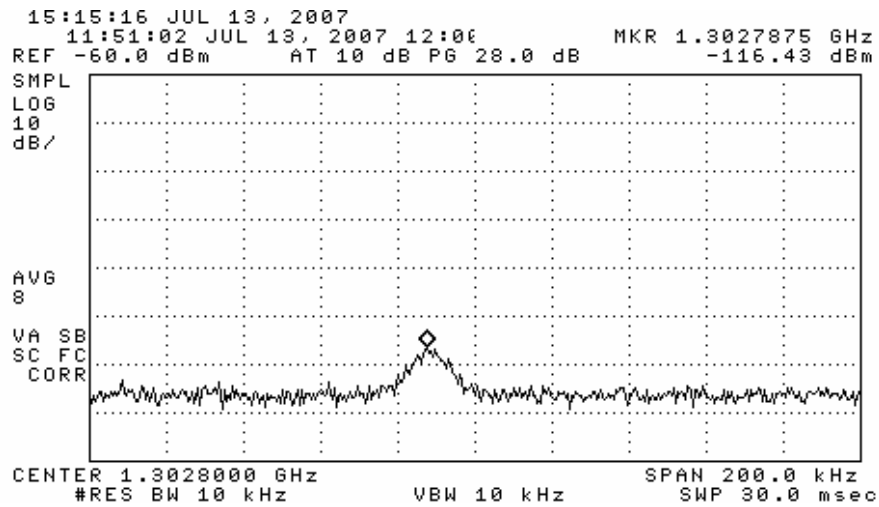
Figure 6.1. Relative receiver emissions (2 x LO and 4 x LO).
