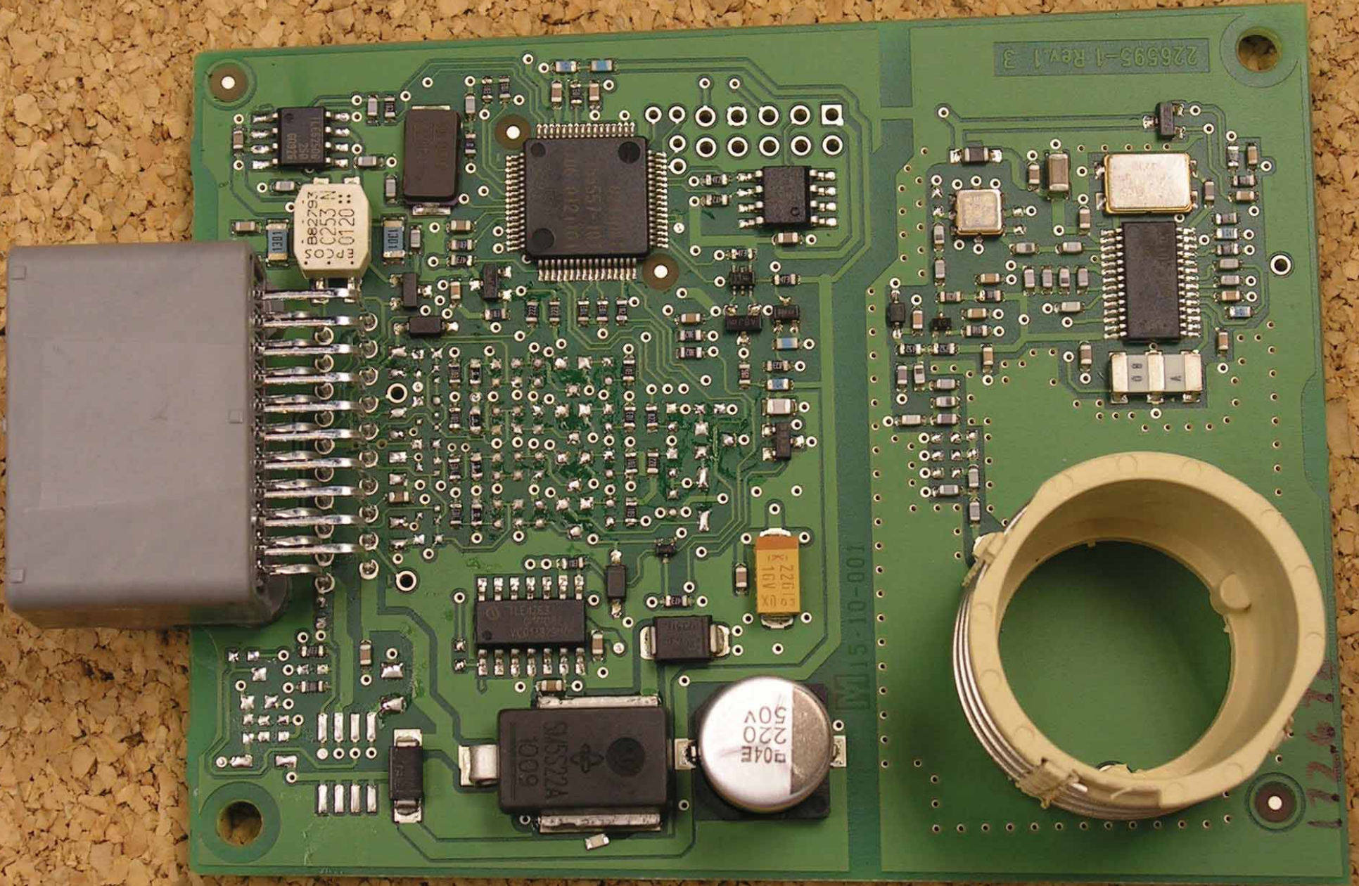
PCB (top)
