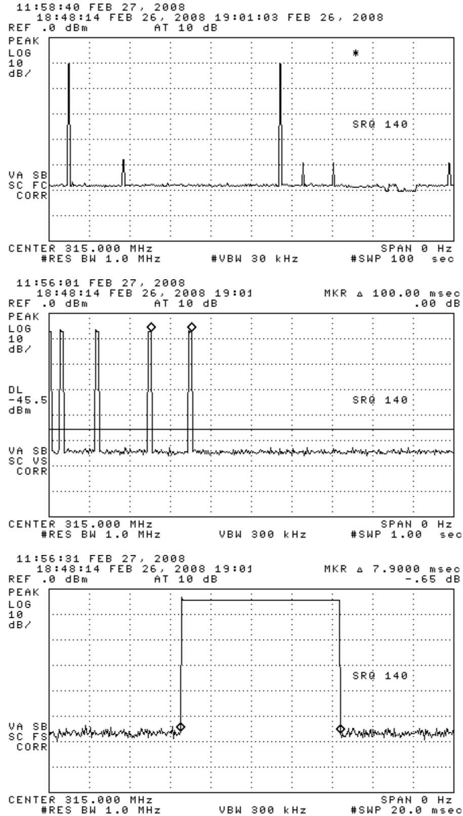
Figure 6.1(a). Transmissions modulation characteristics: (top) response to periodic interrogation, (center) transmitted words, (bottom) single FSK word.
