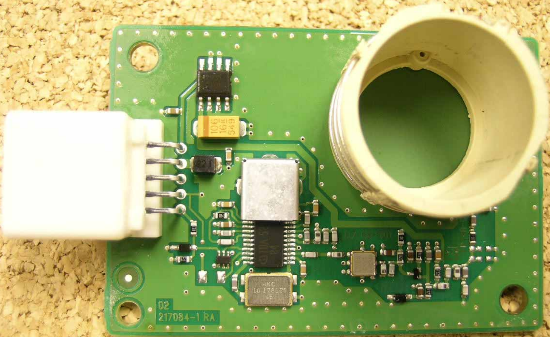
PCB (top)
