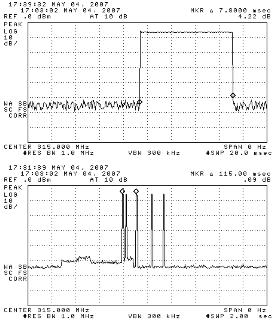
Figure 6.1(b). Transmissions modulation: (top) tx. pulse width, (bottom) two pulses/100ms worst case.
