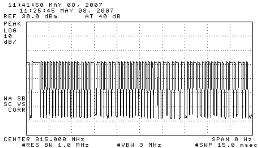
Figure 6.1(a). Transmissions modulation characteristics: (top) duration plot, (center) expanded transmission, (bottom) expanded word.
