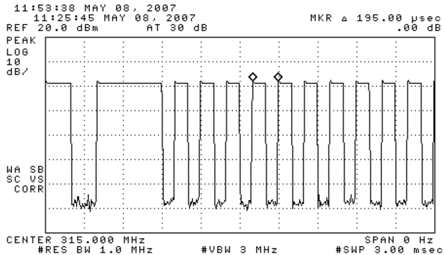
Figure 6.1(b). Transmissions modulation characteristics: (top) wake bit, (center) second wake bit, (bottom) expanded data.
