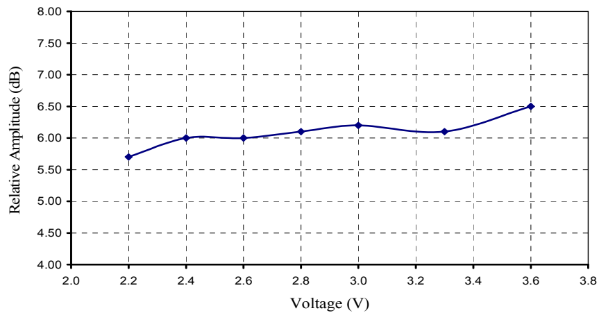
Figure 6.4. Relative emissions at 315 MHz vs. supply voltage (pulsed emission).
