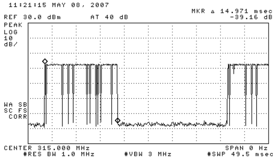
Figure 6.1(a). Transmissions modulation characteristics: (top) 10 sec. verification, (center) complete transmission, (bottom) expanded word.
