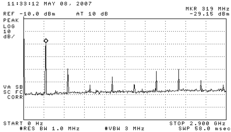
Figure 6.2. Emission spectrum of the DUT (pulsed emission).
