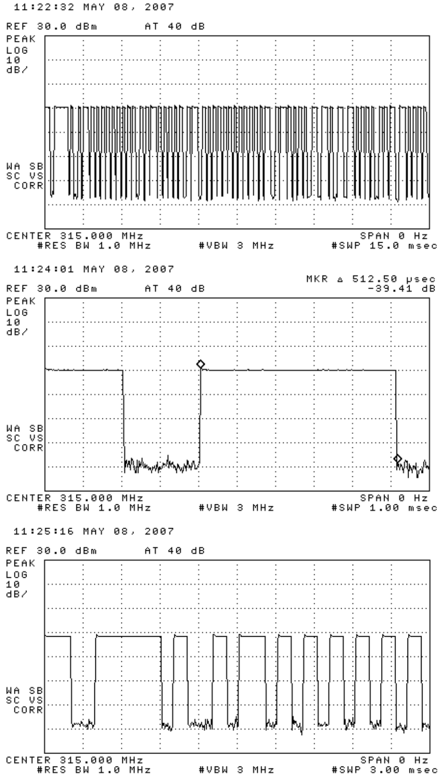
Figure 6.1(b). Transmissions modulation characteristics: (top) expanded word, (center) wake bits, (bottom) following Manchester data.
