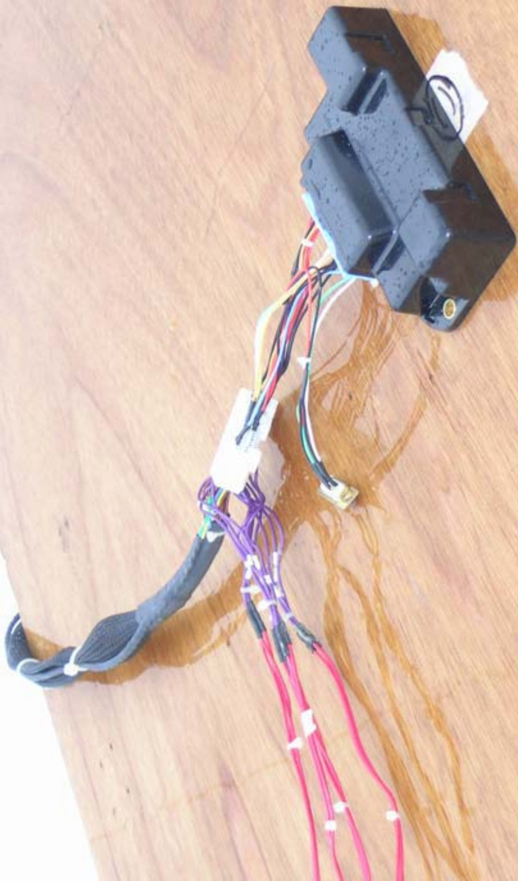
DUT on OATS (close-up)
