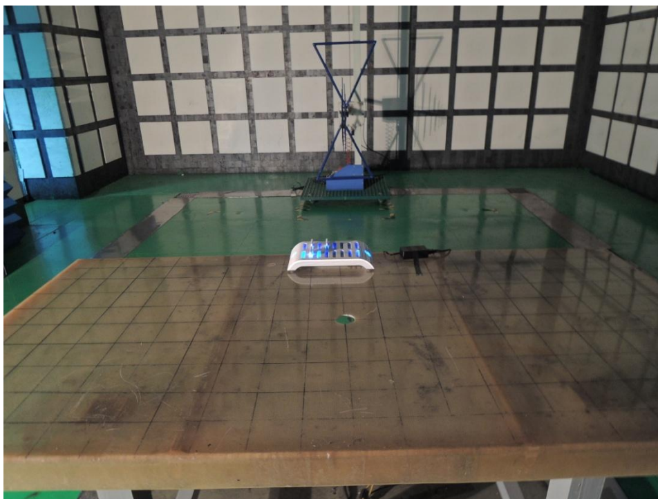
Radiation emission (below 1G)
