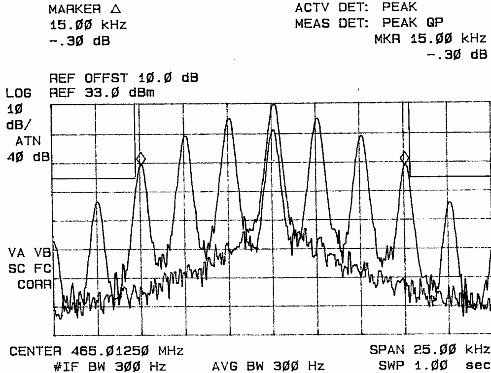
Figure four Occupied Band Width Audio tone (Wideband).
