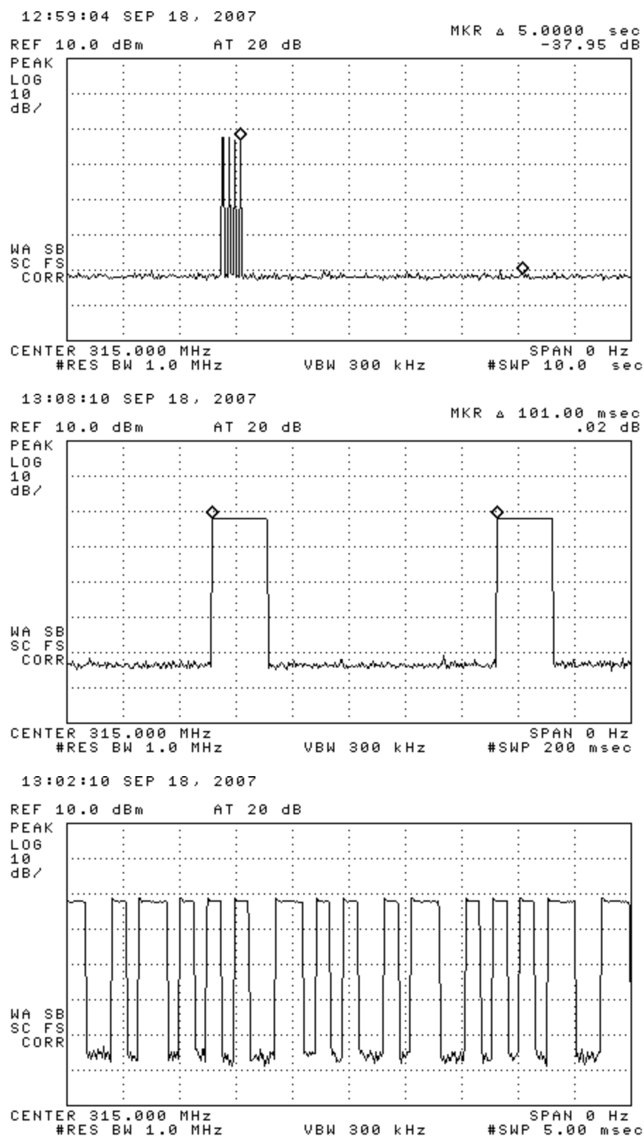
Figure 6.1(a). Transmissions modulation characteristics: (top) single button press, (center) expanded period, (bottom) expanded word.
