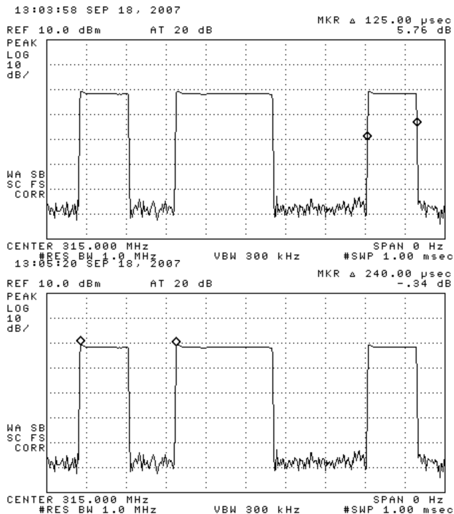
Figure 6.1(b). Manchester characteristics: (top) width, (bottom) period.
