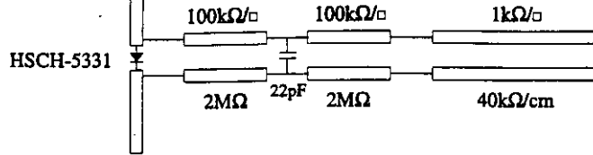
Fig. 3. Equivalent circuit representation of the probe.
