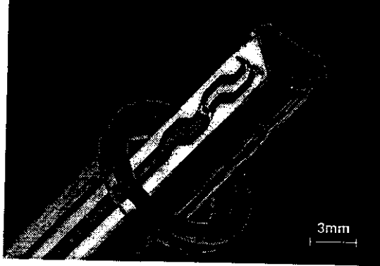
Fig. 1. Tip of the E-field probe. The tip encapsulation has been removed. One 3 mm long dipole and the diode can be seen. In the center of the core is the opening for a built-in optical proximity sensor.
