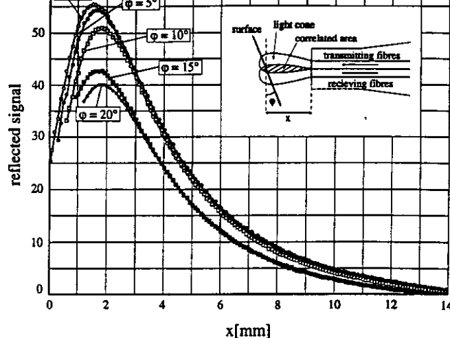
Fig. 10. Response of the surface detector as a function of the distance ( x ) from the surface.
