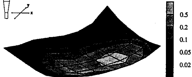
Fig. 8. Distribution of the SAR component normal to the probe axis in the shell phantom measured with a commercial mobile phone.
