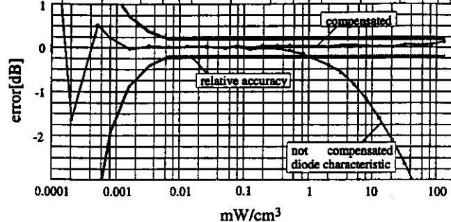
Fig. 12. Deviation from linearity. The line with the dark symbols are the values after compensation of the diode compression. The data was obtained from measurement at 900 MHz in the TEM cell (ifi 110).
