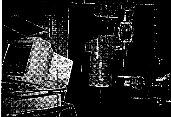
Fig. 1. Laboratory set up including robot, probe, data acquisition electronics, phantom and PC.
