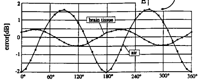
Fig. 7. Deviation from isotropy of the probe with triangular design in air at 2500 MHz (above an open waveguide R26) and in brain tissue equivalent solution (900MHz), whereas the E-field was rotated in a plane through the probe axis.
