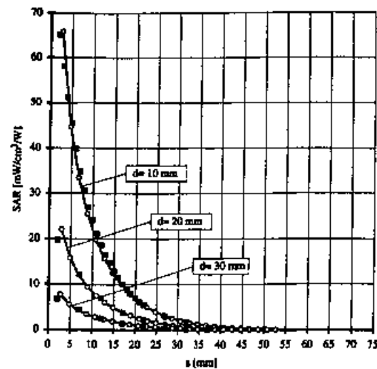
Fig. 8. SAR assessed by E-field (small empty symbols) and temperature measurement (big full symbols) at 1.8 GHz in brain-simulating liquid ( \epsilon_r = 40.5 and \sigma = 1.75 mho/m). The SAR was normalized on 1 Watt input power. The dipole distances from the body were 10 mm, 20 mm and 30 mm. The conversion factor \gamma was determined to 4.8 \pm 10\% .
