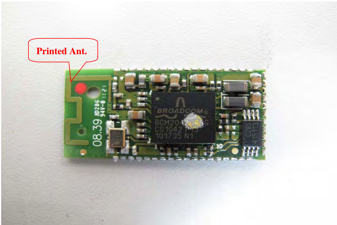
Front view of module
