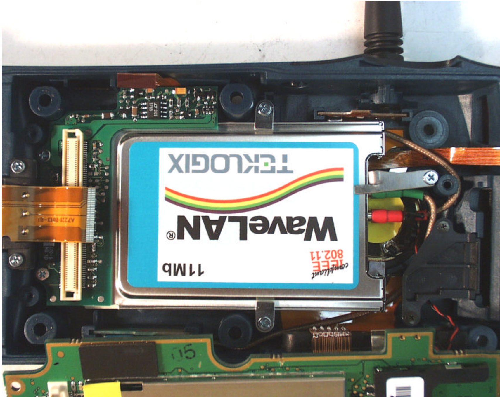
ANNEX 4 - INTERNAL PHOTOGRAPHS OF TEKLOGIX TRX-7431 (FCC ID: GM3WLPC24H) Or Agere 2.4 GHz DSSS 11 Mb PCMCIA Card (FCC ID Number: IMRWLPCE24H) NETPAD + TRX7431 (DSSS Modular Transceiver), Model NETPAD RLAN
