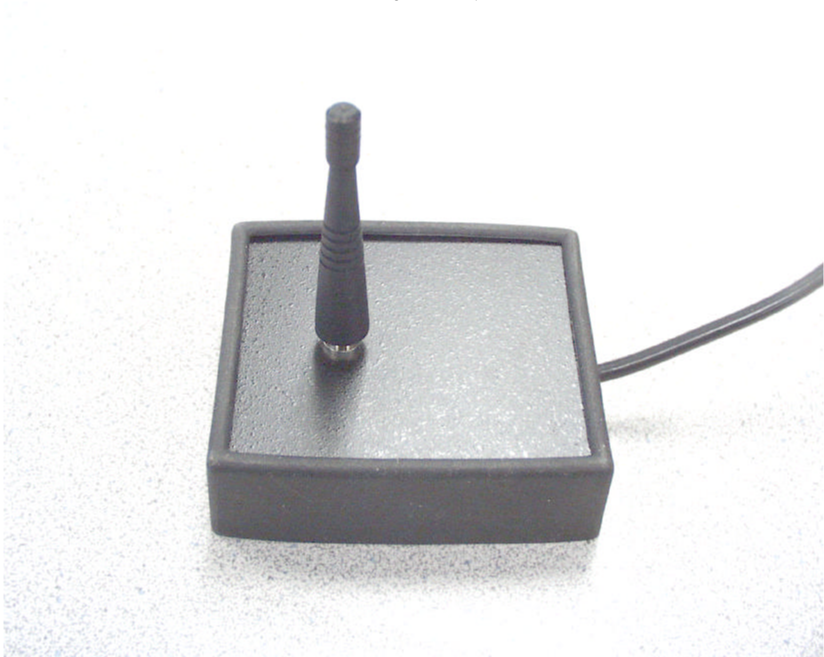
Larsen antenna with reversed thrust SMA connector interface Model: KD MUQ 2400 RSM, Gain: 0 dBi
