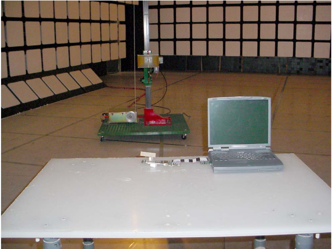
Radiated Emissions at 3 m (RA2040 with Case Integrated PCB Antenna)
